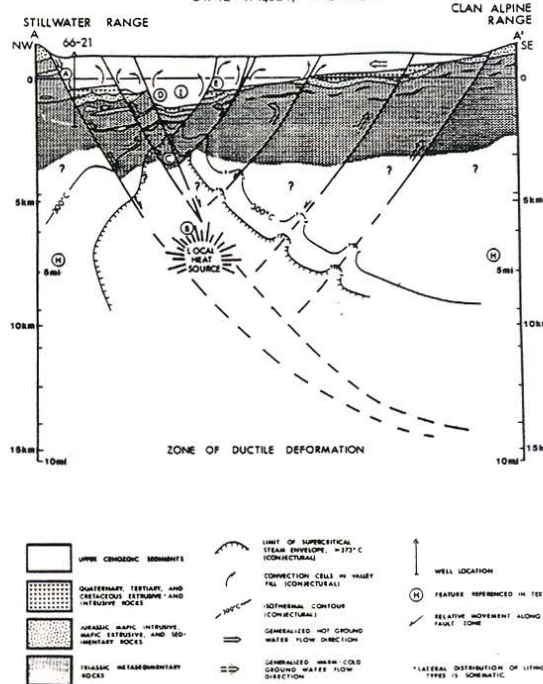
FIGURE 2 GENERALIZED CROSS SECTION* AND CONCEPTUAL GEOTHERMAL CONVECTION SYSTEMS DIXIE VALLEY, NEVADA
