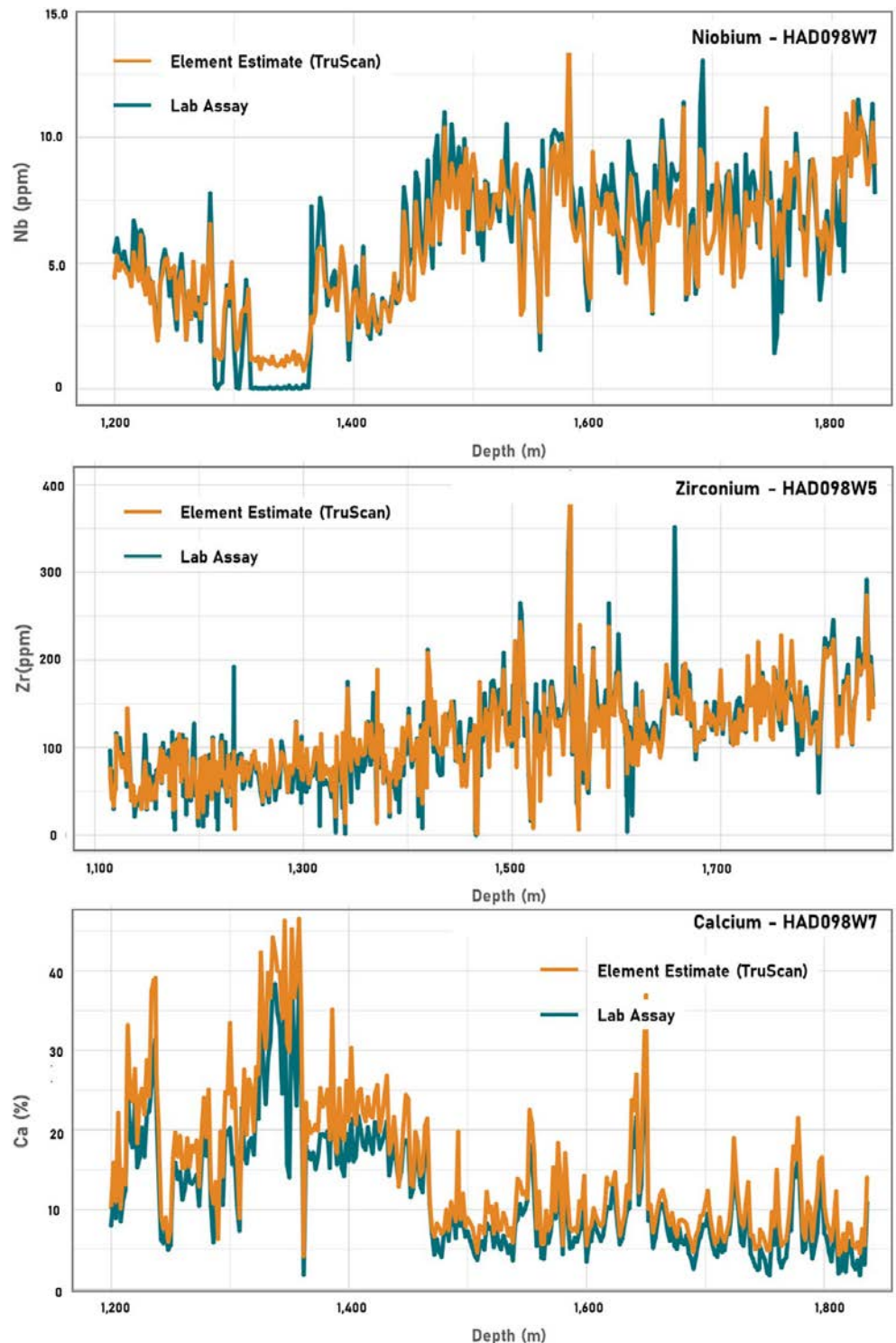
Fig. 10. Example of downhole scatter plots of Nb, Zr, and Ca that compare laboratory assays to values from X-ray fluorescence (XRF) scanning technology (from Havieron, Western Australia). These are elements used by Havieron geologists to log lithology and alteration domains.
