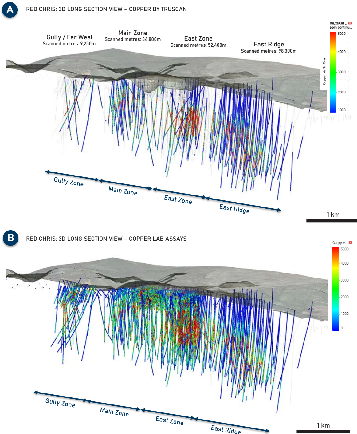
Fig. 6. Distribution of in-field X-ray fluorescence (XRF) scanned drill holes completed at Red Chris (as of May 2023). A. Copper as determined via an in-field XRF scanner is shown on drill traces (gray lines). The determined values are via a process of site-based matrix matching to available multiacid geochemistry. B. Copper determined via lab-based process as has been reported by Newcrest (Newcrest Mining Ltd., 2023).
