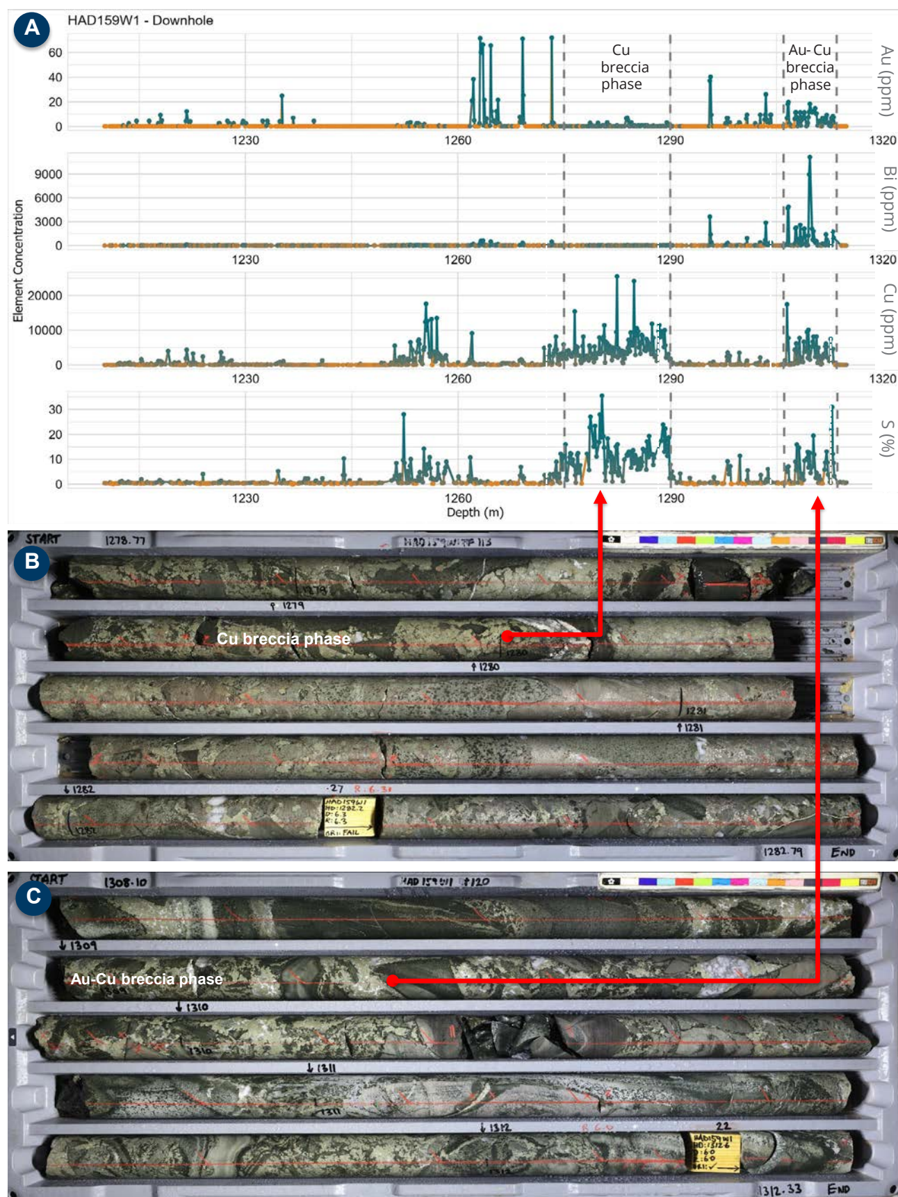
Fig. 9. Example of real-time dashboard used by logging geologists to differentiate near-equivalent metal-bearing breccias (Havieron). A. Two phases of breccia phases can be easily separated using the downhole strip logs. B. Example of the sulfide-bearing breccia with high Cu values compared to C., which is a similar-looking breccia that is more Au rich (inferred from the detectable Au and higher Bi values).
