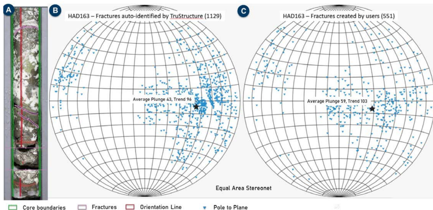
Fig. 11. Machine-driven logging of basic structural data (Havieron). A. Example of automated pickup structural data—both planes and lines—in oriented core photography, with only minor loss in precision of measurement compared to the physical measurement of orientation data. B and C. Geologist/technician-validated automated mapping of structural data can result in larger volumes of robust data compared to fractures mapped via traditional logging. Removal of inconsistencies in manual core logging techniques (including variable experience and training and personal observation bias) means that data collected from all drill core within a deposit can be used in a geotechnical model.
