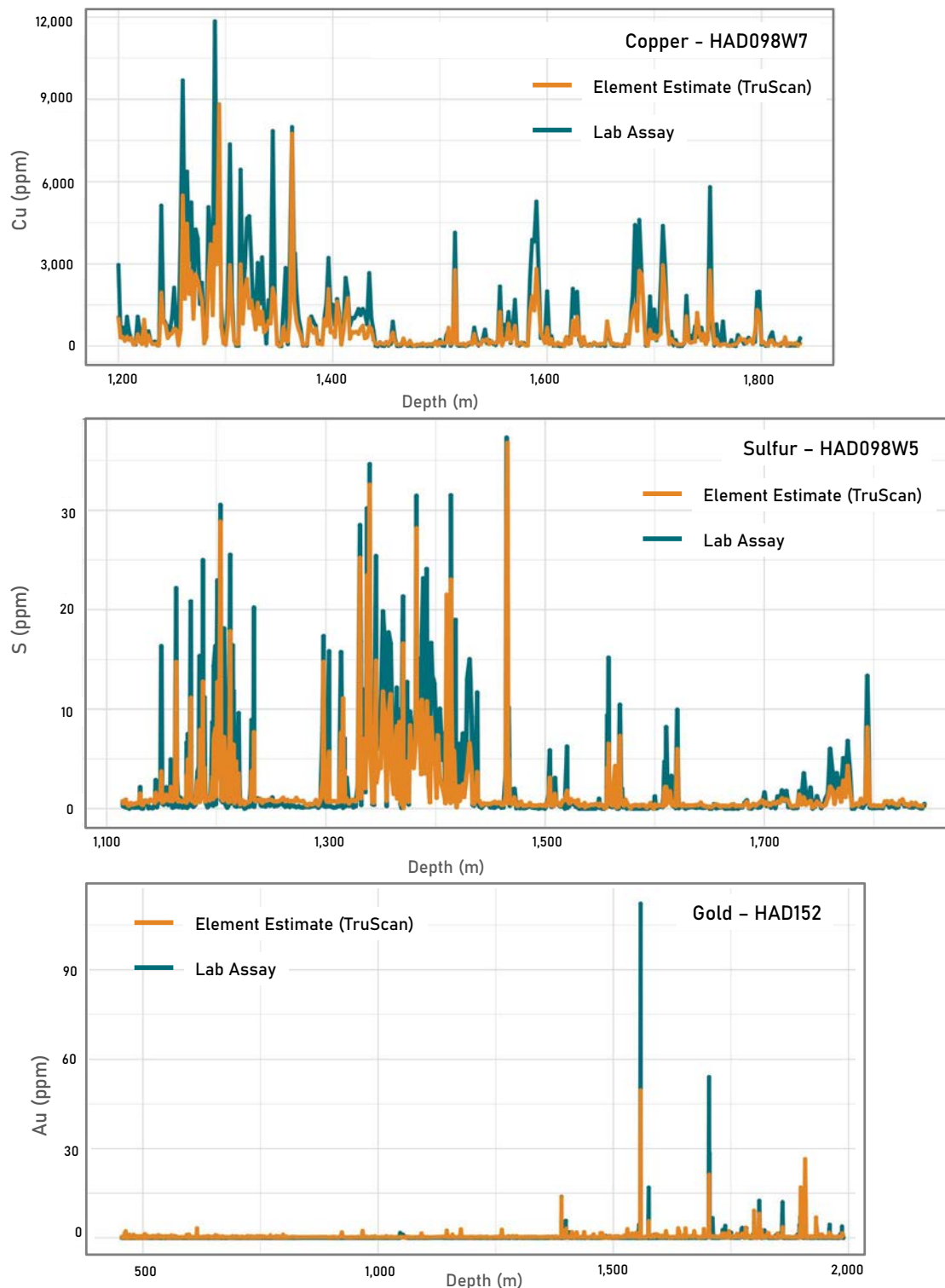
Fig. 8. Example of downhole scatter plots of Cu, S, and Au that compare laboratory assays to values from X-ray fluorescence (XRF) scanning technology (from Haveron, Western Australia). Results presented here are elements used by Haveron geologists to log mineralization zones. Although considered a problematic analysis via in-field XRF technology, a single downhole plot of Au is shown.
