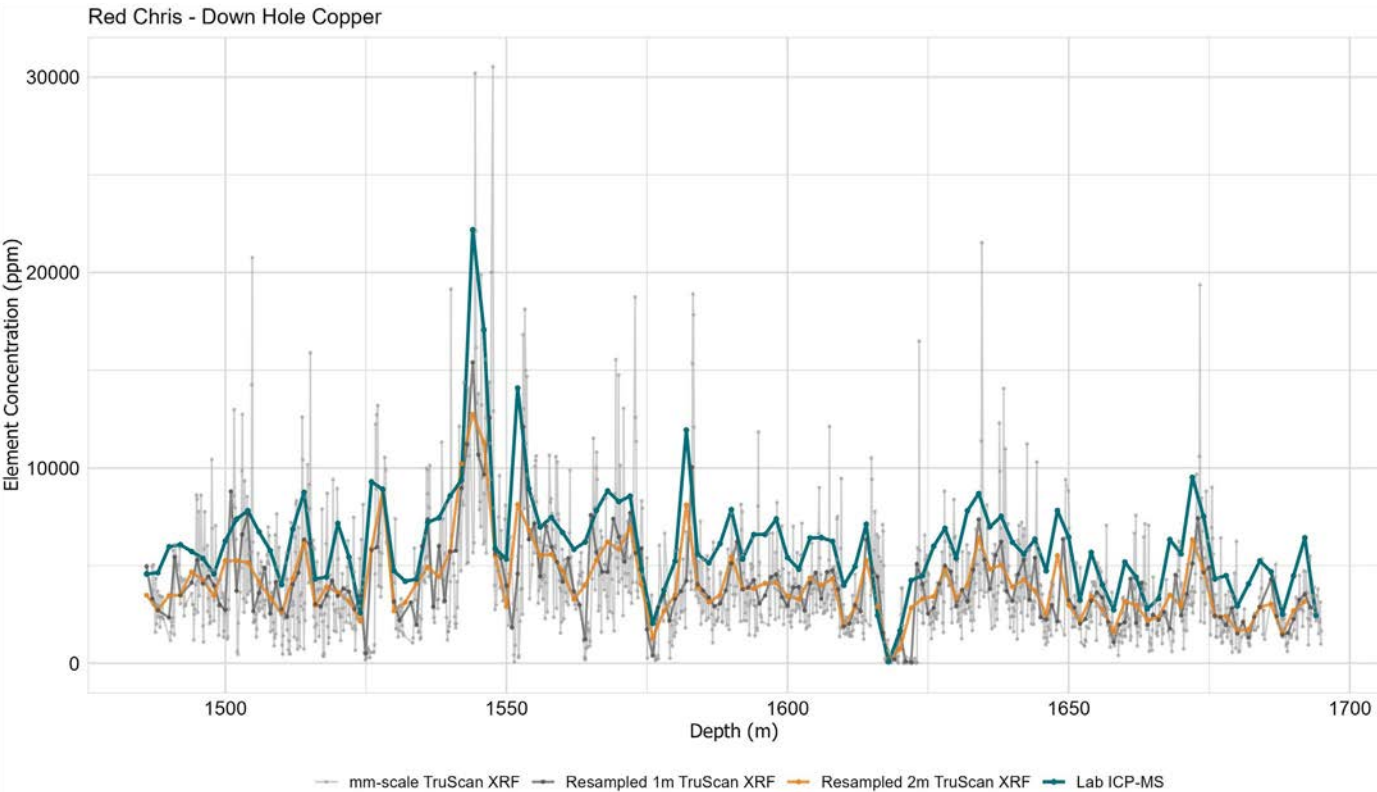
Fig. 4. Example of downhole X-ray fluorescence (XRF) scanner Cu versus lab-based Cu values (Red Chris). Shown here is a comparison between different subsets of the line scan XRF data (millimeter versus meter sample intervals); this highlights the sensitivity of the XRF scanner to heterogeneity within the sample when the millimeter-scale XRF Cu values are compared to meter-scale intervals. The narrow sampling window, combined with the dense sampling, results in spikes of Cu when the beam scans sulfide-bearing veins versus disseminations and/or silicate minerals in the groundmass. ICP-MS = inductively coupled plasma-mass spectrometry.
