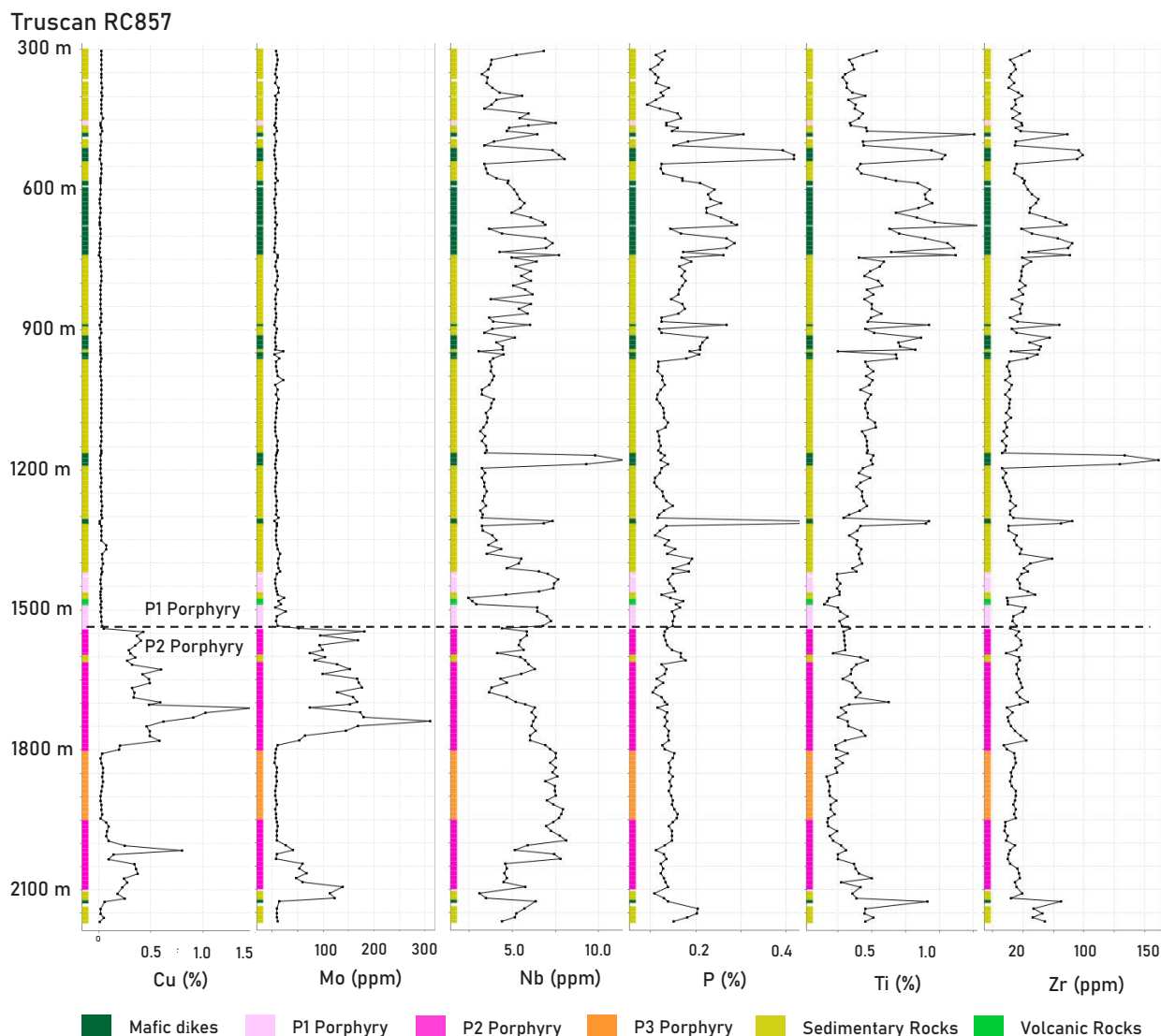
Fig. 5. Example of downhole scatter plot of elements used at Red Chris to help geologists differentiate rock types. The high resolution of the scanning helps geology teams pick the contacts of the porphyry phases (e.g., P1 and P2 contact at 1,520 m). Note the subtle chemical differences in the mafic and felsic dikes in the deposit, which can be differentiated using variations in the concentration of Cu and Mo and Nb, Ti, and Zr.
