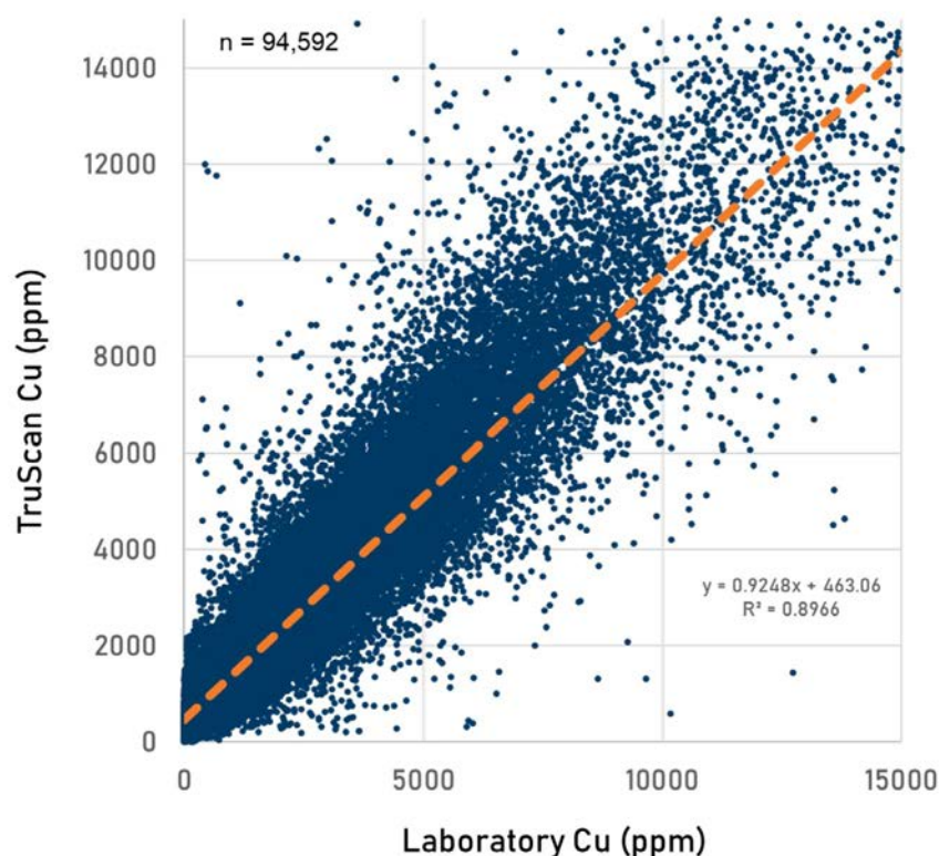
Fig. 7. Correlation between Cu concentrations from laboratory and Cu values from in-field X-ray fluorescence (XRF) scanner.
