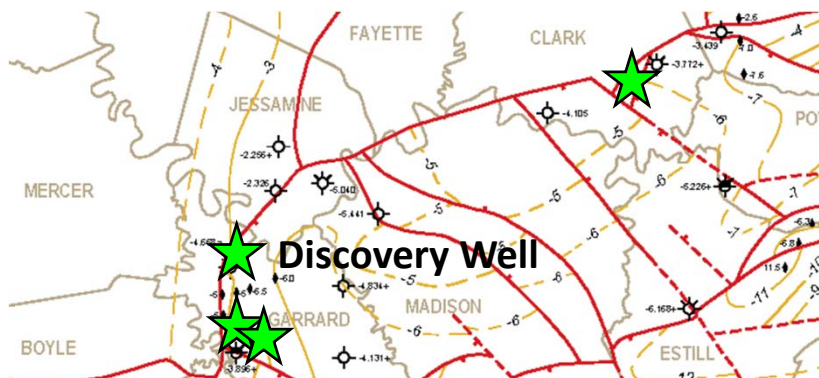
Structural contours on top of central Kentucky Precambrian basement. Green stars are discovery wells with tested high helium-content . From Drahovzal and Noger (1995).
