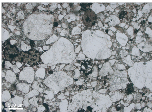
Figure 4 Oil bearing sandstone, uncolored, 2.5x, brightfield transmitted light
