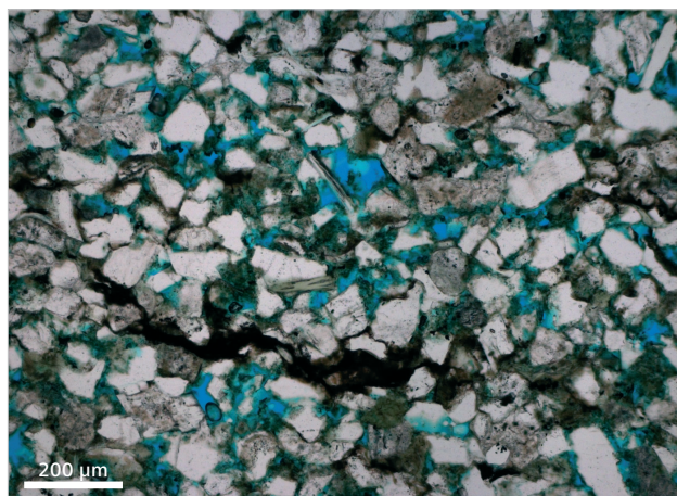
Figure 6 Oil bearing sandstone, blue epoxy dye in pore spaces, 10x, bright-field transmitted light
