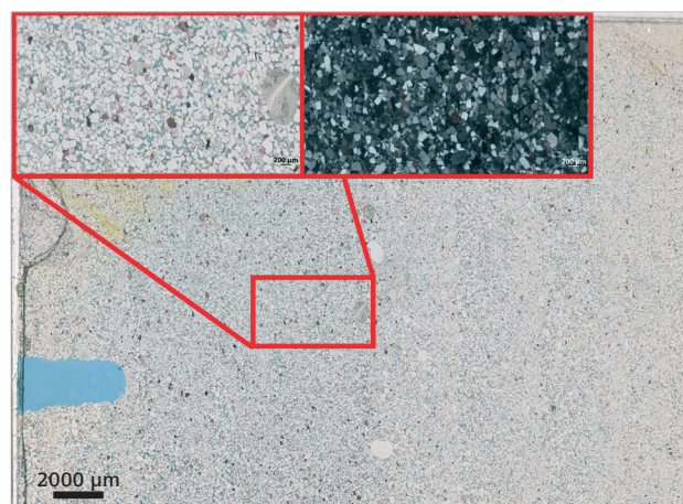
Figure 3 Sandstone, thin section, 20x objective, measured with Axio Scan.Z1 in transmitted light brightfield and polarization.
