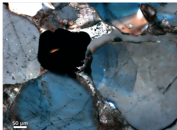
Figure 7 Oil bearing sandstone, 20x pol objective, transmitted polarized light
