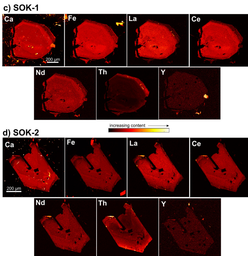
Figure 7. X-ray maps of selected elements for Gruszków and Sokoliki allanite grains. (a) grain GR-1; (b) grain GR-2; (c) grain SOK-1 and (d) grain SOK-2. Black spots in Y X-ray maps are after LA-ICP-MS analyses. The scale is shown only for Al (a,b) and Ca (c,d) maps and is identical for all related images.
