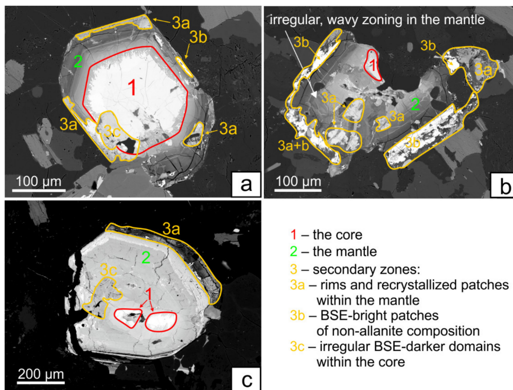
Figure 2. Selected allanite grains with marked textural zones 1 to 3; (a) GR-1, (b) GR-2, and (c) SOK-1.
