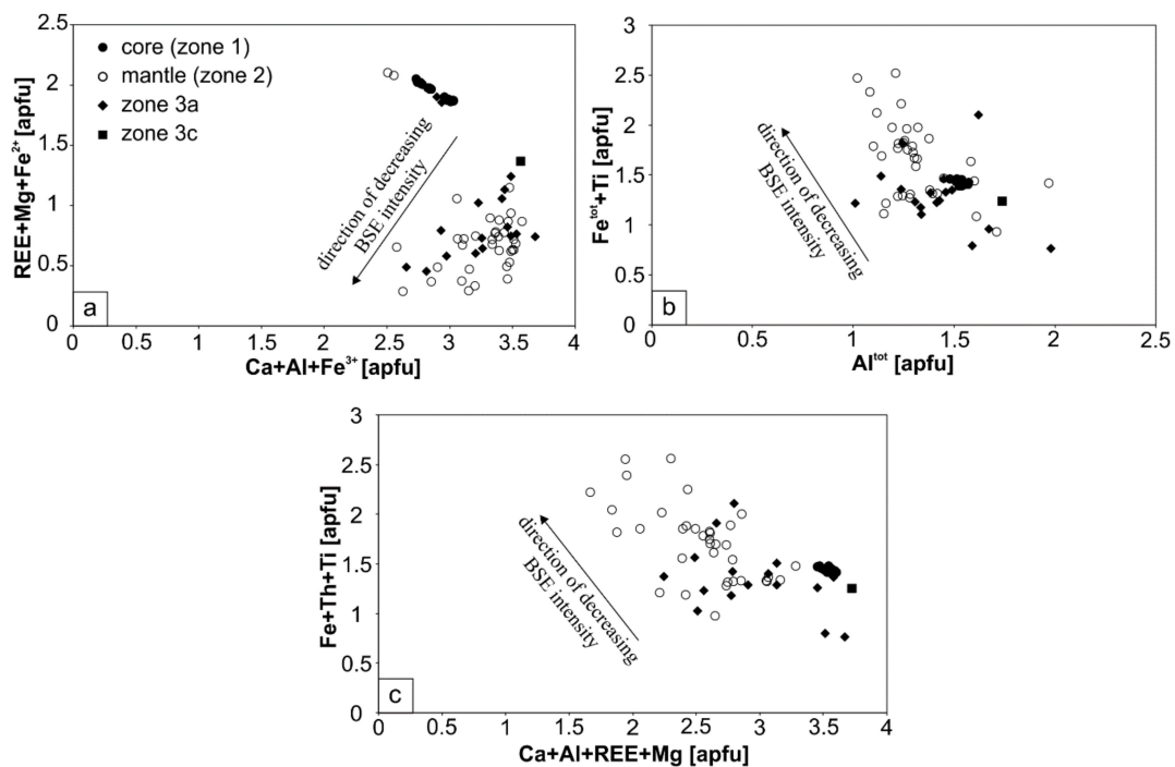
Figure 6. Cationic plots showing possible substitutions in allanite structure: (a) Ca + Al + Fe^{3+} vs. REE + Mg + Fe^{2+} , (b) Al^{tot} vs. Fe^{tot} + Ti, ( Fe^{tot} —total Fe), and (c) Ca + Al + REE + Mg vs. Fe + Th + Ti.
