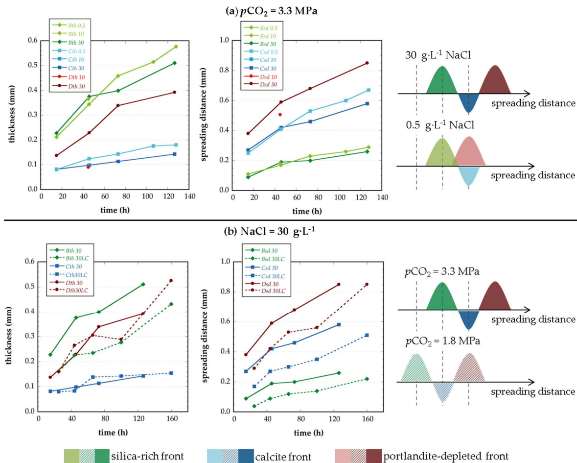
Figure 6. Salinity (a) and p\text{CO}_2 (b) effect on the distribution and dimension of the reaction fronts in the reacted cement samples.
