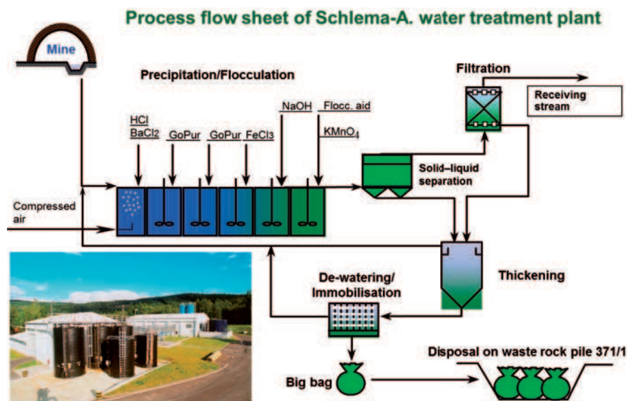
FIG. 7.21. 226 Ra removal in the course of complex water treatment at the Schlema WTP By BaCl 2 precipitation and flocculation using GoPur.
