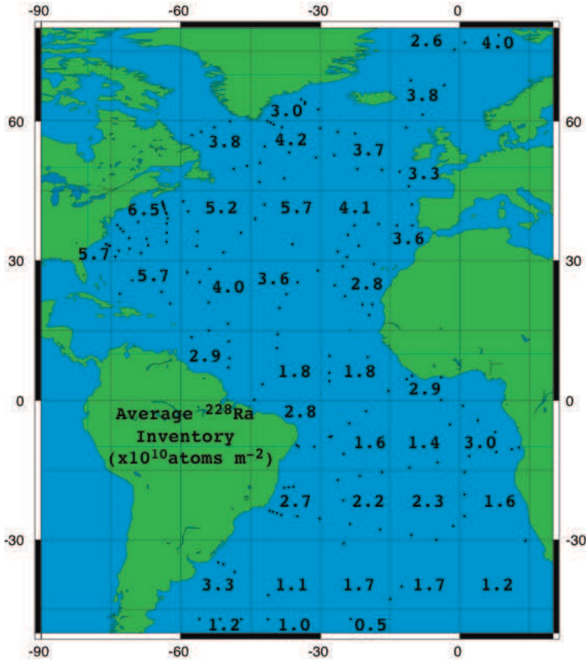
FIG. 7.14. The inventory of ^{228}\text{Ra} ( \times 10^{10} atoms/ \text{m}^2 ) in the upper 1000 m of the Atlantic Ocean based on data collected from 1981–1989. The points show the distribution of stations that were used to calculate ^{228}\text{Ra} inventories. All stations within each 15^\circ \times 15^\circ box were averaged to yield a bin average, shown as a number in each box. The bin averages were then averaged to yield a grand average for the upper Atlantic. The grand average was multiplied by the surface area of the Atlantic to estimate the total ^{228}\text{Ra} inventory in the upper Atlantic (adapted from Moore et al. [7.30]).
