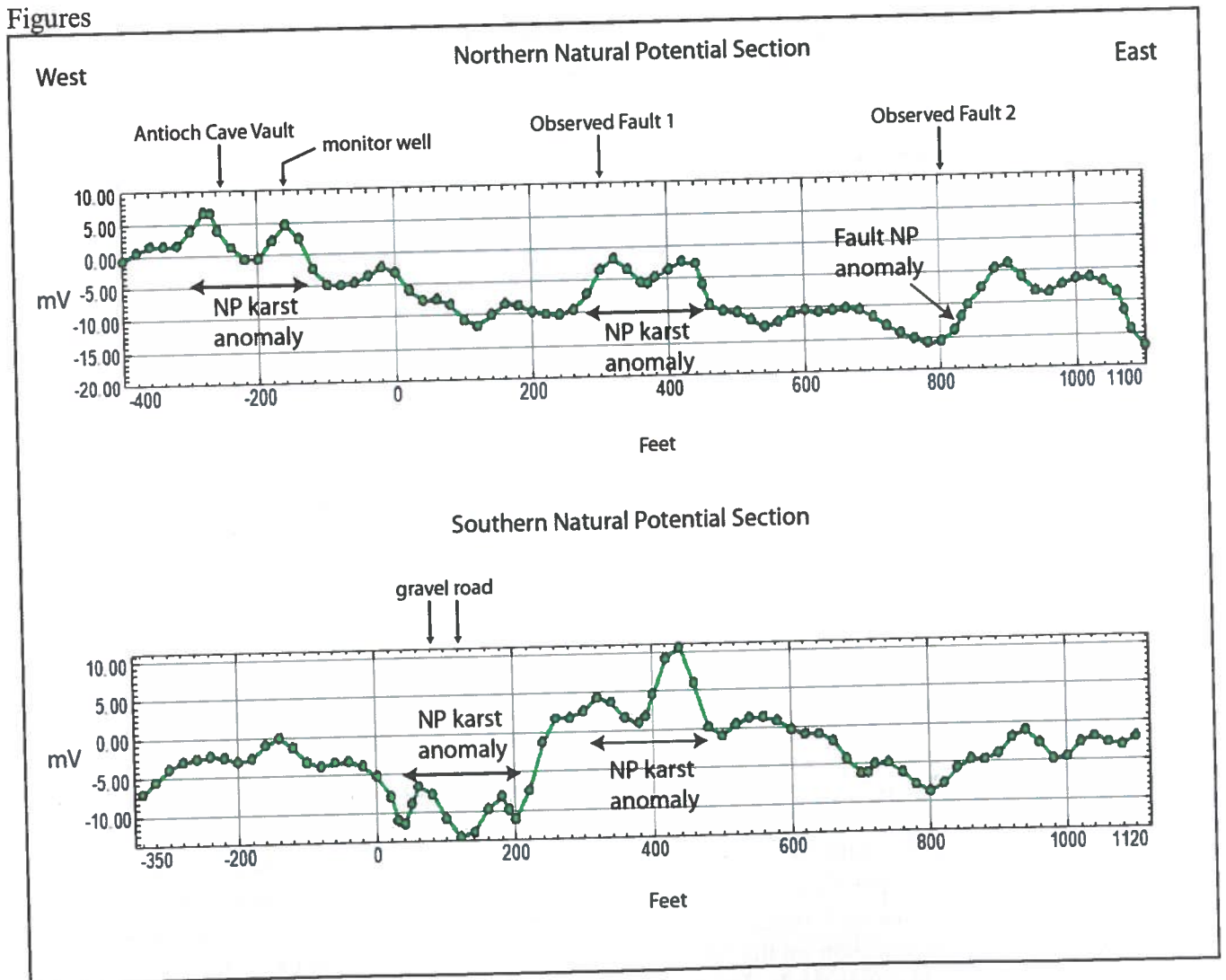
Figure 7. Natural potential data along the northern and southern banks of the Onion Creek. Note the locations of two significant faults observed in Figure 3. Significant NP anomalies are marked on both profiles. One of the NP anomalies located at station -160 ft along the northern bank of the Onion Creek was drilled down to 220 feet. Significant voids were encountered during the drilling.
