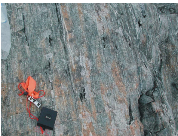
Figure 5 - Interbedded (and deformed) mafic to intermediate bedded tuffaceous units, western shore of McIntock Lake.
