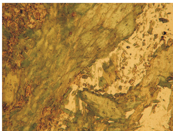
Figure 11 - Photomicrograph of mafic unit. Note feathery actinolite (plane polarized light: width of field of view 6 mm).
