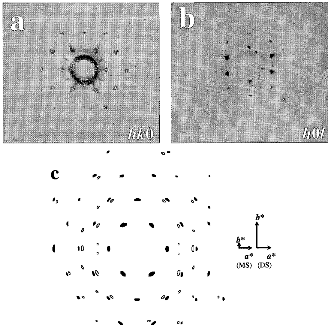
FIG. 6. Precession photographs of crystal schoc after heating in air at 120°C for one hour (a) hk0 photograph; (b) h0l photograph; (c) Representation of the hk0 precession photograph in (3a) with weak diffraction spots enhanced. The pattern indicates the intergrowth of two phases, one with an \alpha - \text{UO}_2(\text{OH})_2 -type sheet: "dehydrated schoepite" (phase 1, filled spots), and one with a structural sheet that may resemble that of metaschoepite (phase 2, hollow spots). Reciprocal axes are indicated at right and labeled "DS" for phase 1 and "MS" for phase 2.
