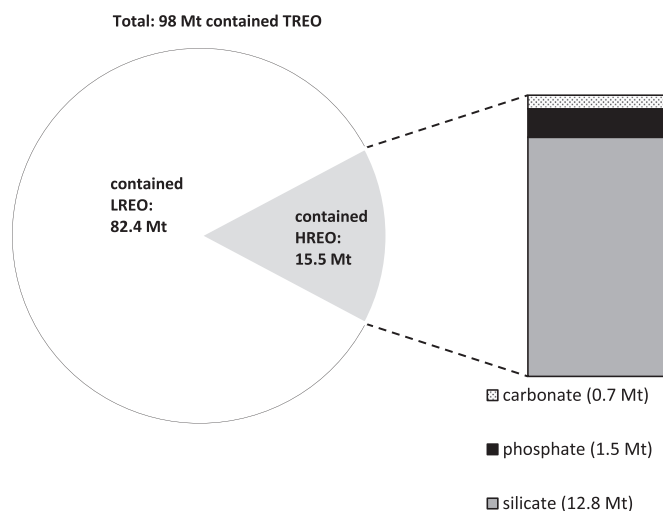
Fig. 7. The total of 98 Mt TREO defined during the REE exploration boom consist mainly of LREO and a smaller fraction of HREO. The contained HREO (15.5 Mt) are strongly concentrated in resources that have silicates as the main REE ore mineral (Table A2).
