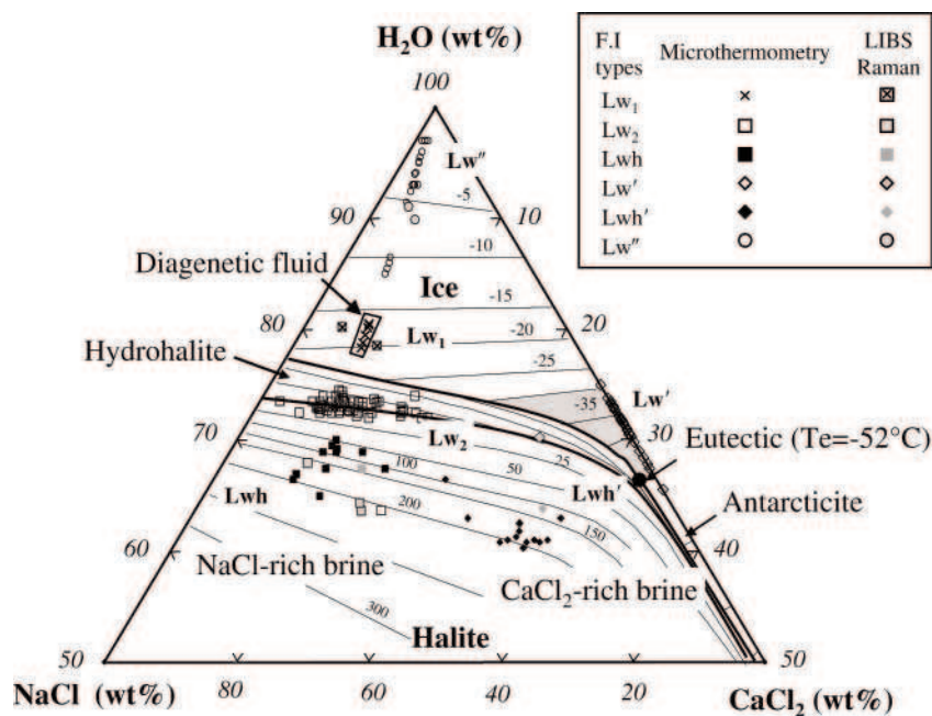
FIG. 8. H_2O -NaCl- CaCl_2 phase diagram with data points issued either from microthermometry or from combined Raman and LIBS analyses for all fluid inclusions types. This diagram shows that most fluid inclusions distribute within two main compositional fields (NaCl- and CaCl_2 -rich brines) and that a series of data points correspond to a series of Lw_1 and Lw'' inclusions (dilute fluids showing evidences of mixing or contamination with a more saline end member).
