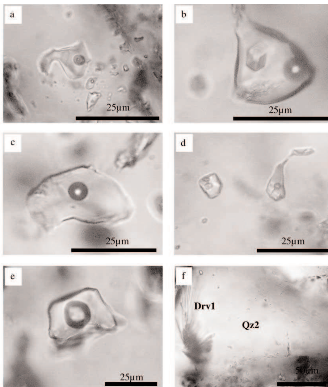
FIG. 5. Petrographic characteristics of the different fluid inclusions observed in the McArthur River deposit. (a) Lw, (b) Lwh, (c) Lw', (d) Lwh', (e) Lw'', (f) fluid inclusions in Qz2 close to dravites (Drv1).
