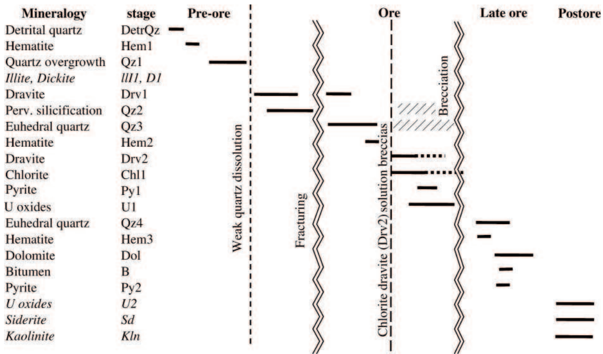
FIG. 3. Summary of the mineral paragenesis in the McArthur River uranium deposit determined from field and thin section observations of the samples from the present study. Data from Kotzer and Kyser (1995) are indicated in italics. Full lines = mineral growth; cross hatch = dissolution. Abbreviations: B = bitumen, Chl = chlorite, D = dickite, Dol = dolomite, Drv = dravite, Hem = hematite, Ill = illite, Kln = kaolinite, Py = pyrite, Qz = quartz, Sd = siderite, U = uranium oxide.
