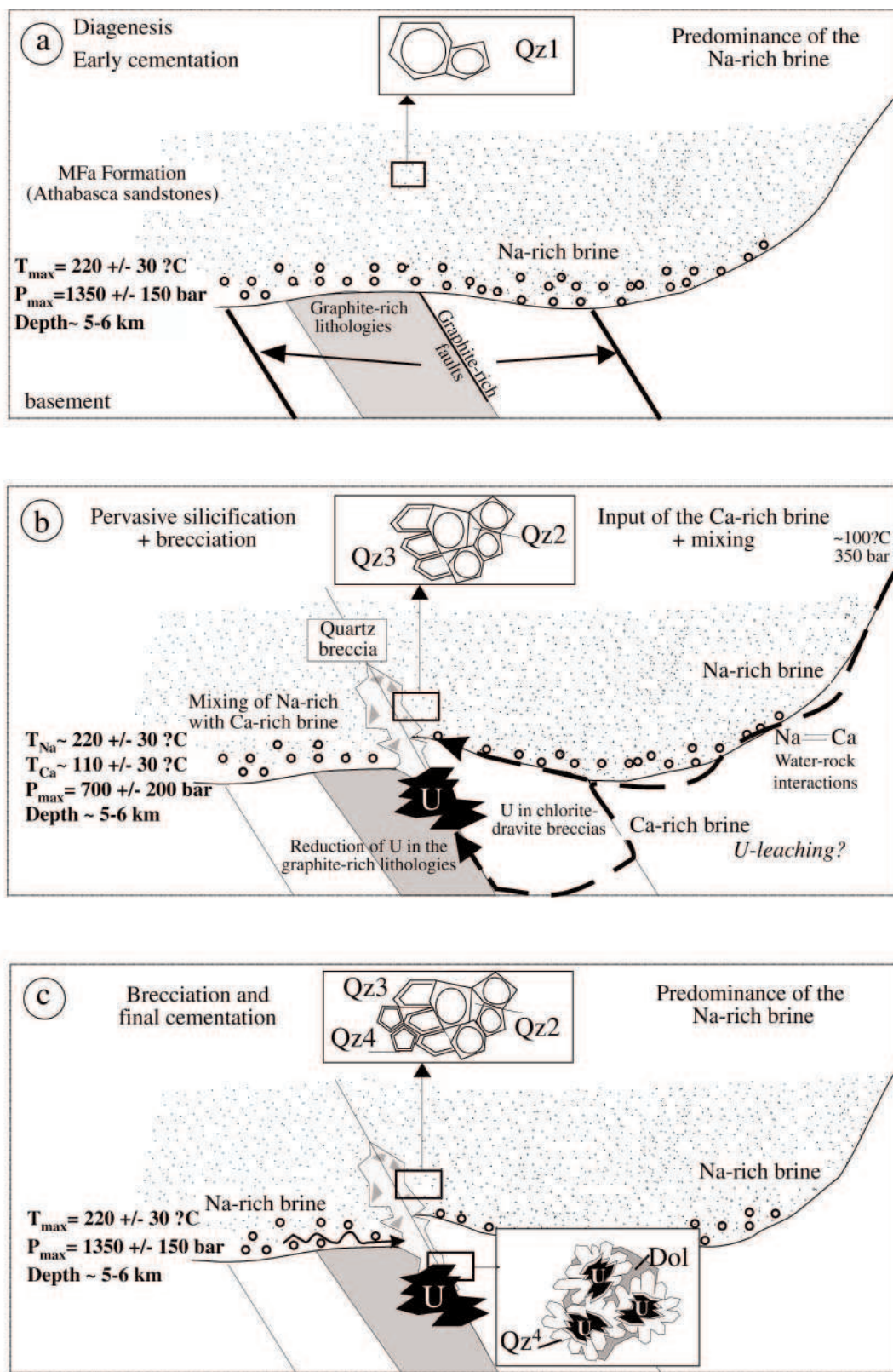
FIG. 10. Schematic representation of fluid circulation and P-T conditions that prevail at the base of the basin at each step of quartz cementation in the McArthur River deposit area and its possible link with the genesis of U mineralization. (a). Early cementation at the bottom of the sandstone formation. (b). Interactions of the Na-rich brine with Ca-rich lithologic units and formation of a Ca-rich brine which subsequently mixed with main Na-rich brines along fault zones (uranium deposition stage). (c). Final cementation of breccias by Na-rich brines.
