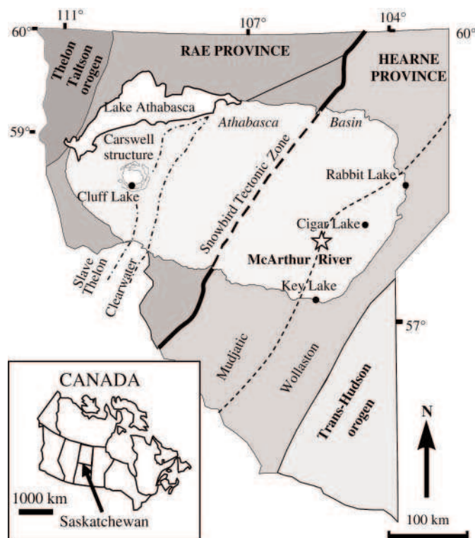
FIG. 1. Location of the main unconformity-type uranium deposits in the Athabasca basin (modified from Ruzicka, 1986).
