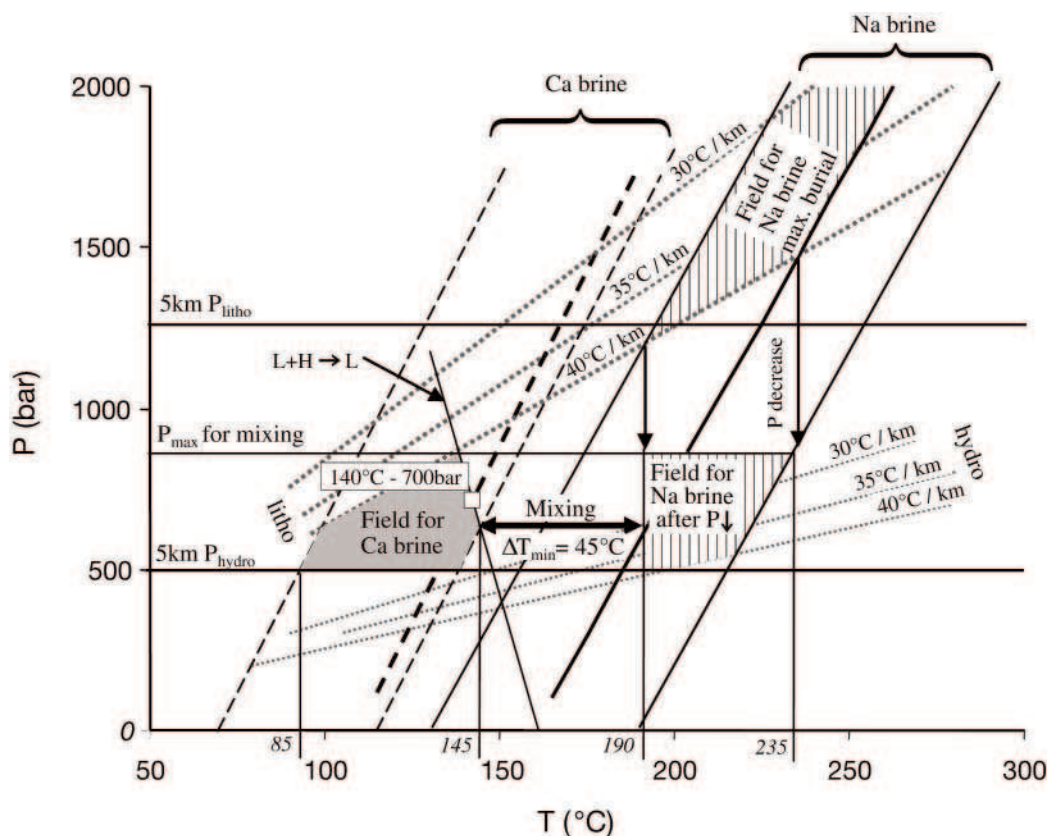
FIG. 9. P-T path model for the NaCl-rich brine and conditions of mixing with the \text{CaCl}_2 -rich brine. Representative isochores (dashed lines) have been drawn for the main ranges of T_h for the two fluid types. The hydrostatic and lithostatic pressures at 5-km depth are reported as well as the hydrostatic and lithostatic gradients calculated for thermal gradients of 30°, 35°, and 40°C/km (dotted lines). The main P-T boxes representative of the trapping conditions of the early brines at the maximum of burial and the trapping of the two main brines are reported in gray.
