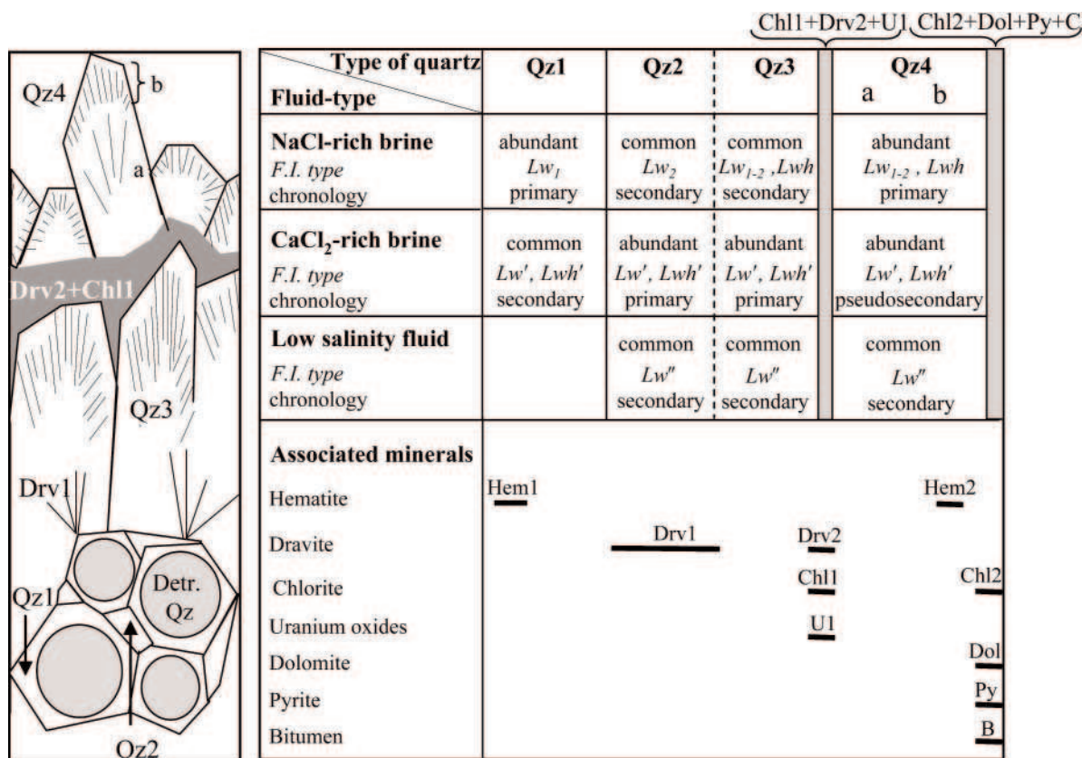
FIG. 6. Chronological and petrographic relationships between the different types of fluid inclusions and the sequence of minerals in the sandstones from the McArthur River deposit. The relative abundance of each fluid type is given as a function of the quartz type in the paragenetic sequence, with indication of the primary or secondary feature of the fluid inclusions and the type of associated mineral. For the quartz Qz4, two stages are distinguished: "a" corresponds to the first growth stage, and "b" to the late growth bands with abundant primary Lw 1-2 and Lwh inclusions. Abbreviations: F.I. = fluid inclusion, Qz = quartz.
