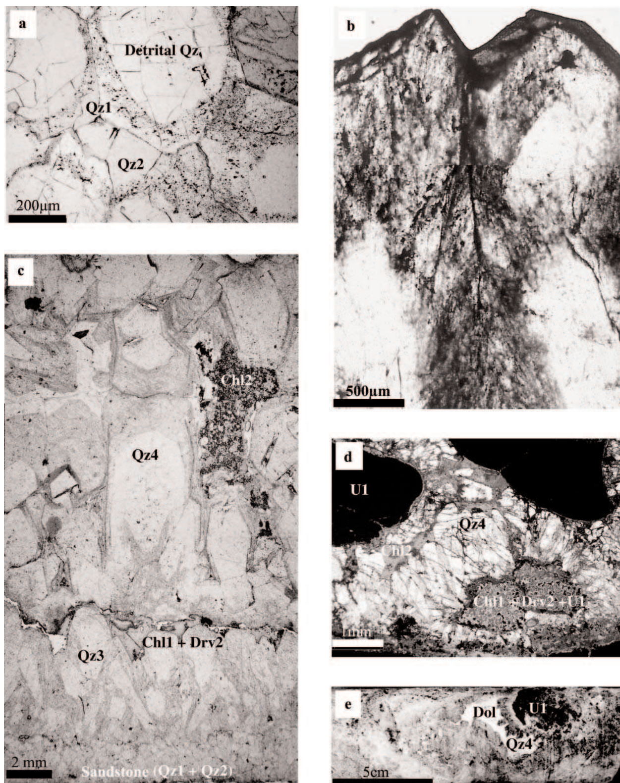
FIG. 4. (a). Sandstone with quartz overgrowths (Qz1) and pervasive silicifications (Qz2); (thin section, transmitted light; Mac 196-529.4m). (b). Primary and pseudosecondary fluid inclusions in euhedral quartz Qz3 in sample H521-71.7m (thick section, transmitted light). (c). Highly silicified sandstone (H521-71.7m), crosscut by a euhedral quartz vein (Qz3) followed by chlorite (Chl1), dravite (Drv2), and euhedral quartz (Qz4) and a second generation of chlorite (Chl2) (thin section, transmitted light). (d). Uranium oxide (U1) in a chlorite (Chl1)-dravite (Drv2) breccia, in turn brecciated and cemented by drusy quartz veins (Qz4) (thin section, transmitted light, sample H393-98.2m). (e). Fragment of pitchblende (U1) in a breccia cemented by quartz (Qz4) and dolomite (Dol) (sample H459-33m).
