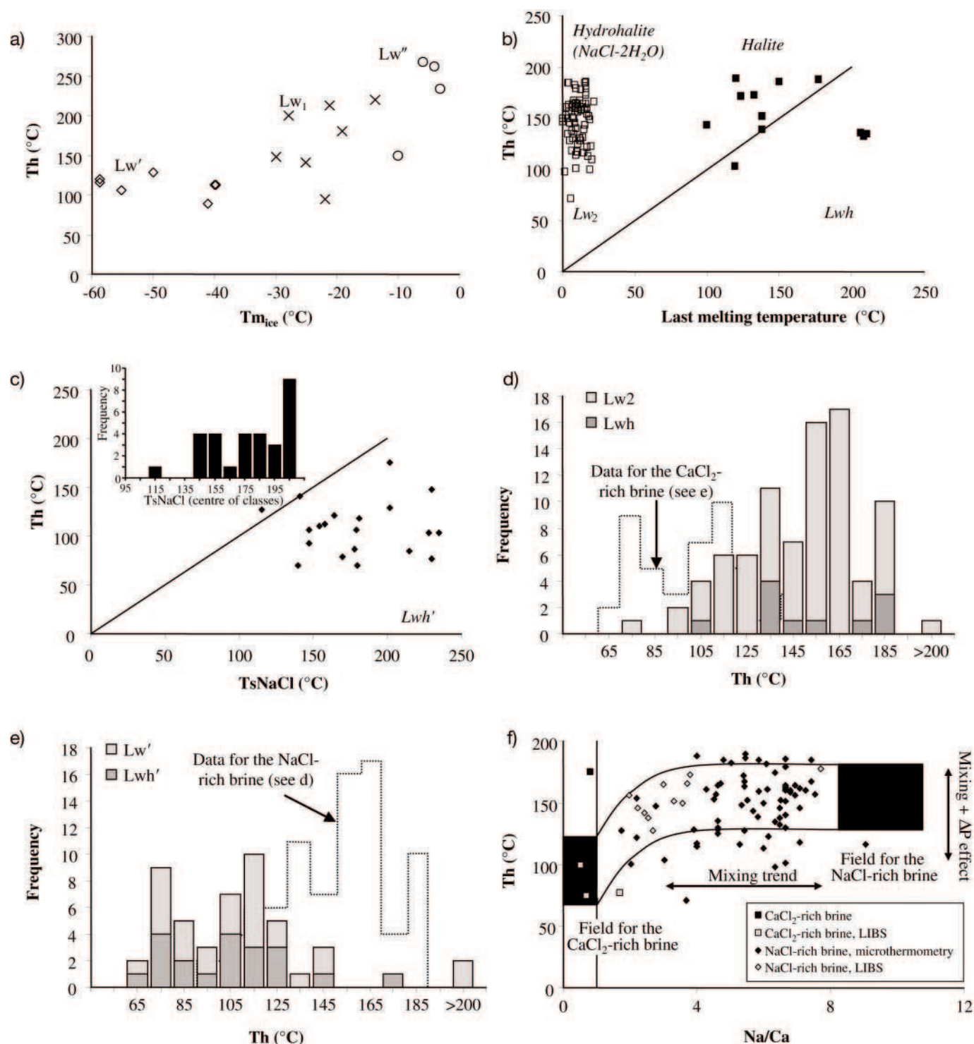
FIG. 7. Microthermometric data. (a). Homogenization temperature ( T_h ) vs. ice-melting temperature ( T_{m(ice)} ) diagram for the liquid-vapor fluid inclusions ( Lw_1 , Lw' , and Lw'' , which correspond to the NaCl-, CaCl 2 -rich brine, and low-salinity fluid, respectively). (b). T_h vs. T_m of the last solid phase for the NaCl-rich brine ( Lw_2 and Lwh inclusions). (c) T_h vs. T_{m(NaCl)} diagram and histogram of T_{m(NaCl)} for the CaCl 2 -rich Lwh' brine inclusions. (d). T_h histogram for the NaCl-rich Lw_2 and Lwh fluid inclusions. (e). T_h histogram for the CaCl 2 -rich Lw' and Lwh' brine inclusions. (f). T_h vs. Na/Ca diagram for the NaCl- and CaCl 2 -rich brine inclusions. Gray data points correspond to LIBS data, whereas black data points correspond to the estimates deduced from the phase transition temperatures in an H_2O -NaCl-CaCl 2 phase diagram. The fields corresponding to the predominant T_h values are reported for the NaCl- and the CaCl 2 -rich brines.
