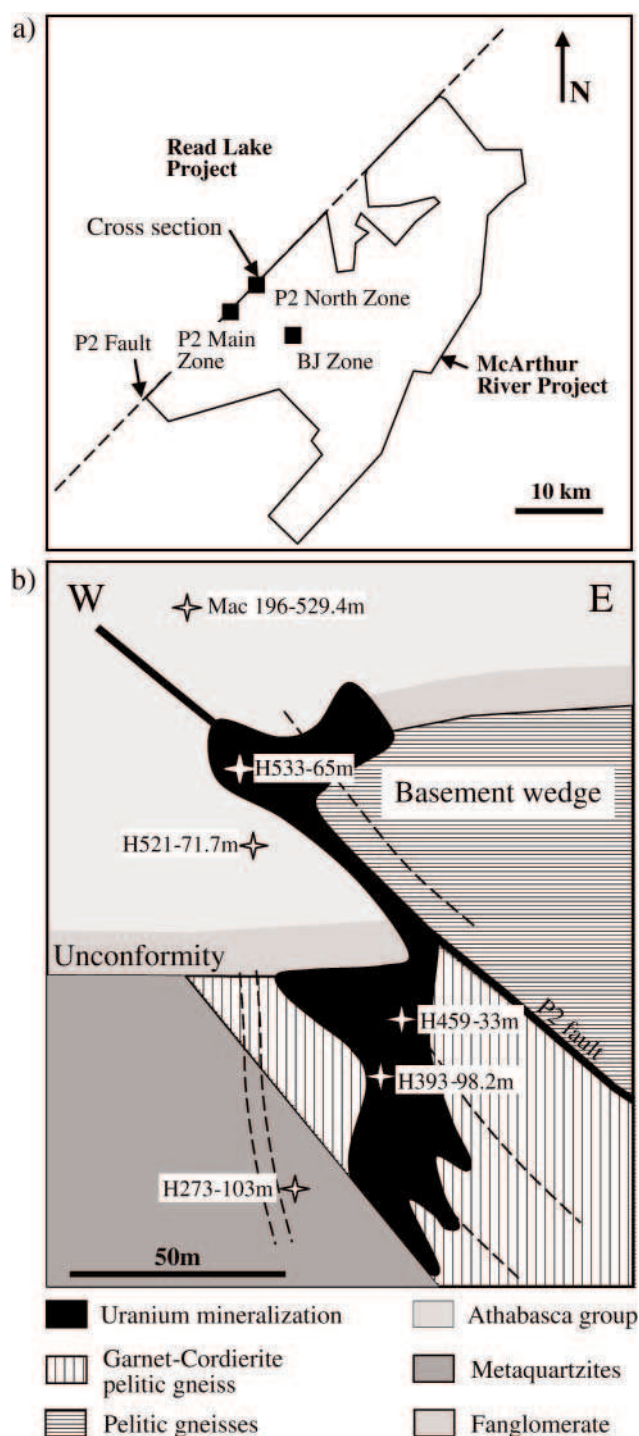
FIG. 2. (a). Location of the McArthur River area. (b). Schematic cross section of the P2 North zone (McArthur River deposit), showing the projection of the approximate location of most of the studied samples (modified from Thomas et al., 2000).
