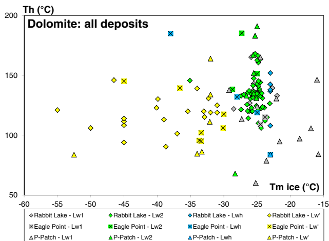
Fig. 5 Ice melting temperature ( T_m ice)-homogenization temperature ( T_h ) relationships of the dolomite-hosted Athabasca fluid inclusions for the Rabbit Lake, Eagle Point, and P-Patch deposits
