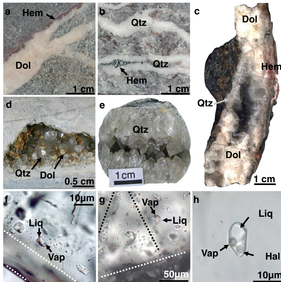
Fig. 2 Examples of fluid inclusion hosting quartz and dolomite veins studied in this work. a Hematite-dolomite vein cross-cutting a biotite-rich gneiss (sample H1935-8, Eagle Point). b Quartz±hematite veins cross-cutting a hematite-rich gneiss (sample ERC5-922.0, Shea Creek). c Quartz-dolomite vein cross-cutting a hematite-rich gneiss (sample RBL2Qz, Rabbit Lake). d Quartz-dolomite vein cross-cutting “bleached” (illite-chlorite-dravite alteration) gneiss (sample CX52-1, Millennium). e Quartz vein cross-cutting “bleached” gneiss (sample P48-5, P-Patch). f Primary two-phase (liquid+vapor) fluid inclusions aligned along a dolomite growth band (highlighted by white dashed lines ). g Cluster of primary and pseudosecondary two-phase (liquid+
