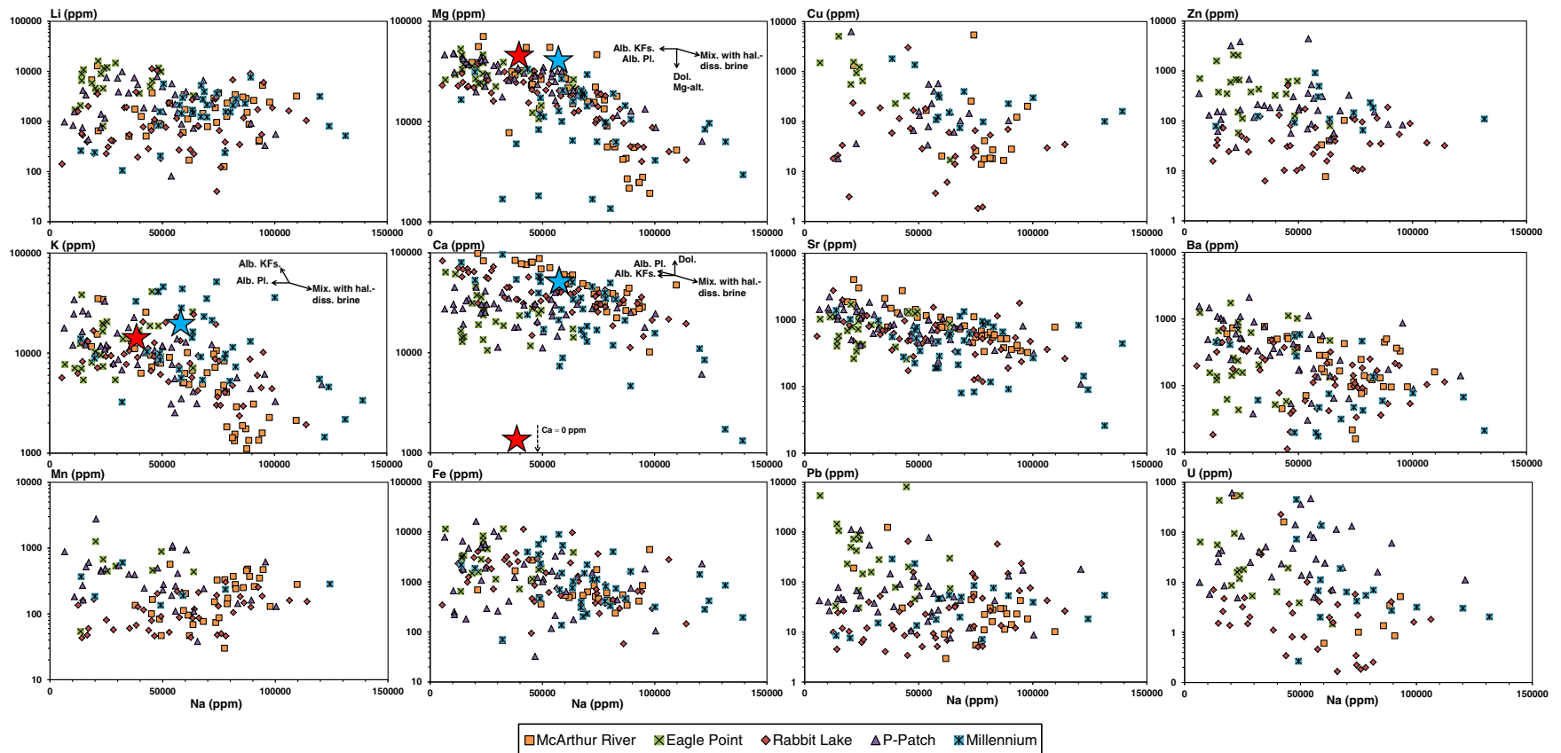
Fig. 7 LA-ICP-MS data for individual quartz-hosted fluid inclusions from the Rabbit Lake, P-Patch, Eagle Point, Millennium, and McArthur River deposits. Data for McArthur River after Richard et al. (2010). Stars indicate the possible composition of epsomite-saturated evaporated seawater from which the NaCl-rich and CaCl 2 -rich brines originated. Red stars (MgSO 4 seas) after Fontes and Matray (1993). Blue stars (CaCl 2 seas) after Lowenstein and Timofeeff (2008). Arrows indicate the expected directions of compositional shifts for the following reactions: Mix. with hal.-diss. brine mixing with halite-dissolution brine, Dol. dolomitization of calcite, Alb. Pl. albitization of plagioclase, Alb. KFs. albitization of K-feldspar, Mg-alt. Mg alteration (sidoite, dravite)
