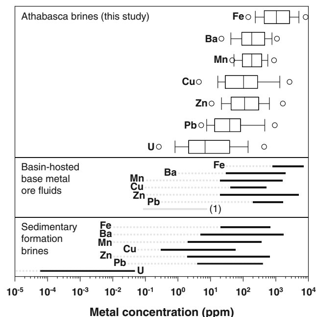
Fig. 10 Ranges of metal concentrations in sedimentary formation brines (from boreholes, after Carpenter et al. 1974; Kraemer and Kharaka 1986; Kharaka et al. 1987; Banner et al. 1990; Connolly et al. 1990; Stueber and Walter 1991; Land and Macpherson 1992; Pluta and Zuber 1995; Hodge et al. 1996; Hitchon et al. 2001; Aquilina et al. 2002) and ore fluids from basin-hosted base metal (Pb, Zn, Ba) deposits (from LA-ICP-MS analysis of fluid inclusions, after Appold et al. (2004); Stoffell et al. (2004); Bouch et al. (2006); Huizenga et al. (2006); Piqué et al. (2008); Stoffell et al. (2008); Sánchez et al. 2009; Wilkinson et al. 2009; Appold and Wenz (2011)) and Athabasca fluid inclusions (this study). Boxplots show 5th and 95th percentiles (symbols), 10th and 90th percentiles (whiskers), 25th and 75th percentiles (box edges), and the median (inner bar). (1) Typical limits of detection for LA-ICP-MS analysis of metals in fluid inclusions. Black solid lines represent the ranges of the highest values for metal concentrations in each of the selected studies. Gray dotted lines represent the lower ranges of metal concentrations in the selected studies
