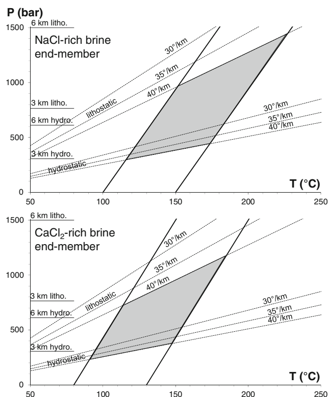
Fig. 9 Possible P-T reconstruction of the Athabasca brines under static geothermal gradient condition. Representative isochores have been drawn from the most representative range of homogenization temperatures (Th) in both quartz and dolomite. The possible P-T field for the NaCl-rich brine end-member (i.e., before mixing) is \sim 180 \pm 30 °C and \sim 800 \pm 400 bars. The possible P-T field for the \text{CaCl}_2 -rich brine end-member (i.e., before mixing) is \sim 120 \pm 30 °C and \sim 600 \pm 300 bars. The hydrostatic and lithostatic pressures at 3- and 6-km depth are reported as well as the hydrostatic and lithostatic gradients calculated for thermal gradients of 30, 35, and 40 °C/km
