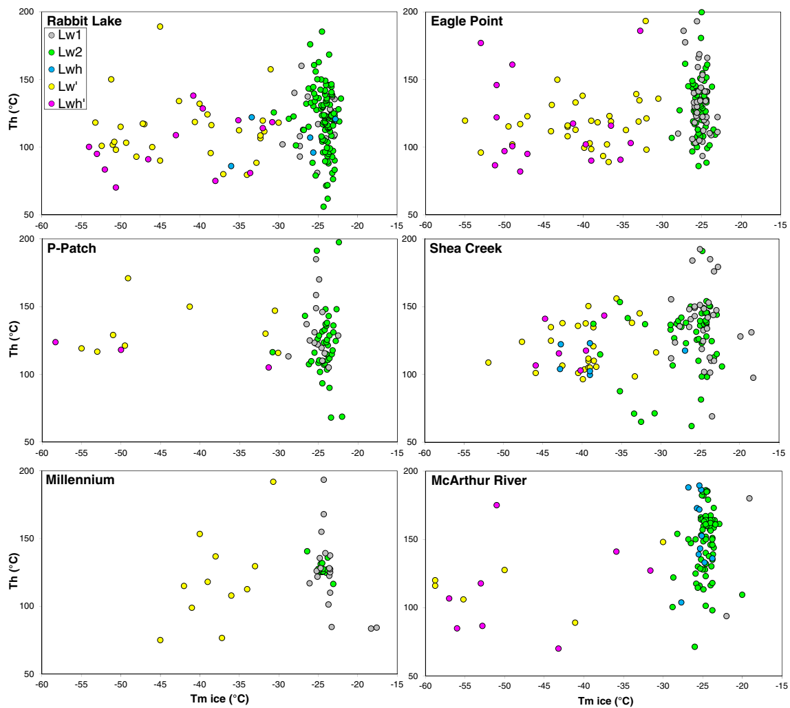
Fig. 4 Ice melting temperature ( T_m ice)-homogenization temperature ( T_h ) relationships of the quartz-hosted Athabasca fluid inclusions for the P-Patch, Eagle Point, Shea Creek, and Rabbit Lake deposits, together with data for the McArthur River deposit from Derome et al. (2005)
