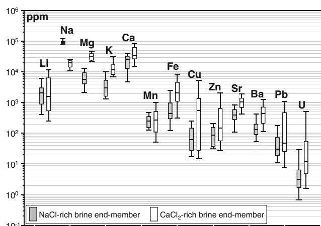
Fig. 8 Ranges of element concentrations for the NaCl-rich brine and \text{CaCl}_2 -rich brine end-members from LA-ICP-MS data. The NaCl-rich brine end-member is defined by fluid inclusions with \text{Na} > 80,000 ppm. The \text{CaCl}_2 -rich brine end-member is defined by fluid inclusions with \text{Na} < 30,000 ppm. Boxplots show 10th and 90th percentiles (whiskers), 25th and 75th percentiles (box edges), and the median (inner bar)
