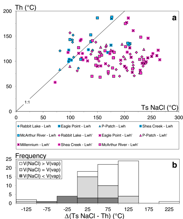
Fig. 6 Homogenization temperature ( Th )-halite dissolution temperature ( Ts\ NaCl )-phase volume relationships of the Athabasca fluid inclusions for the P-Patch, Eagle Point, Shea Creek, and Rabbit Lake deposits, together with data for the McArthur River deposit from Derome et al. (2005). a Ts\ NaCl vs Th for quartz- and dolomite-hosted fluid inclusions. Note that Lwh' inclusions were not found in dolomite. b Distribution of \Delta(Ts\ NaCl - Th) values as a function of the volumetric relationship between NaCl and the vapor phase in the fluid inclusions. V(vap) volume of the vapor phase, V(NaCl) volume of the NaCl phase
