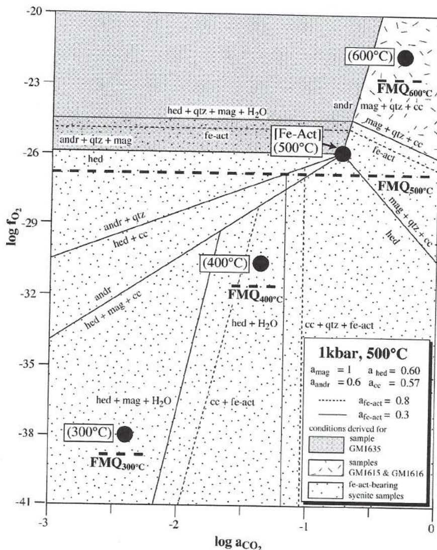
Fig. 13. \log f_{\text{O}_2} - \log a_{\text{CO}_2} diagram (1 kbar) for the system Ca-Fe-Si-O-H-C involving hedenbergite, magnetite, quartz, ferro-actinolite, andradite and calcite. •, position of the invariant point [Fe-Act]; bold dashed lines show the position of the FMQ buffer curve at specified temperatures. The grey, dashed and stippled fields represent the inferred conditions of formation of secondary Ca-mineral assemblages for syenite samples. (See text for further explanation.)
