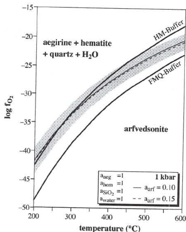
Fig. 14. Log f_{O_2} - T diagram showing the position of reaction (6). The FMQ and HM buffer curves are indicated. The grey field marks the uncertainty if an error of \pm 0.2\% for \Delta fT^0(\text{arf}) is assumed.
