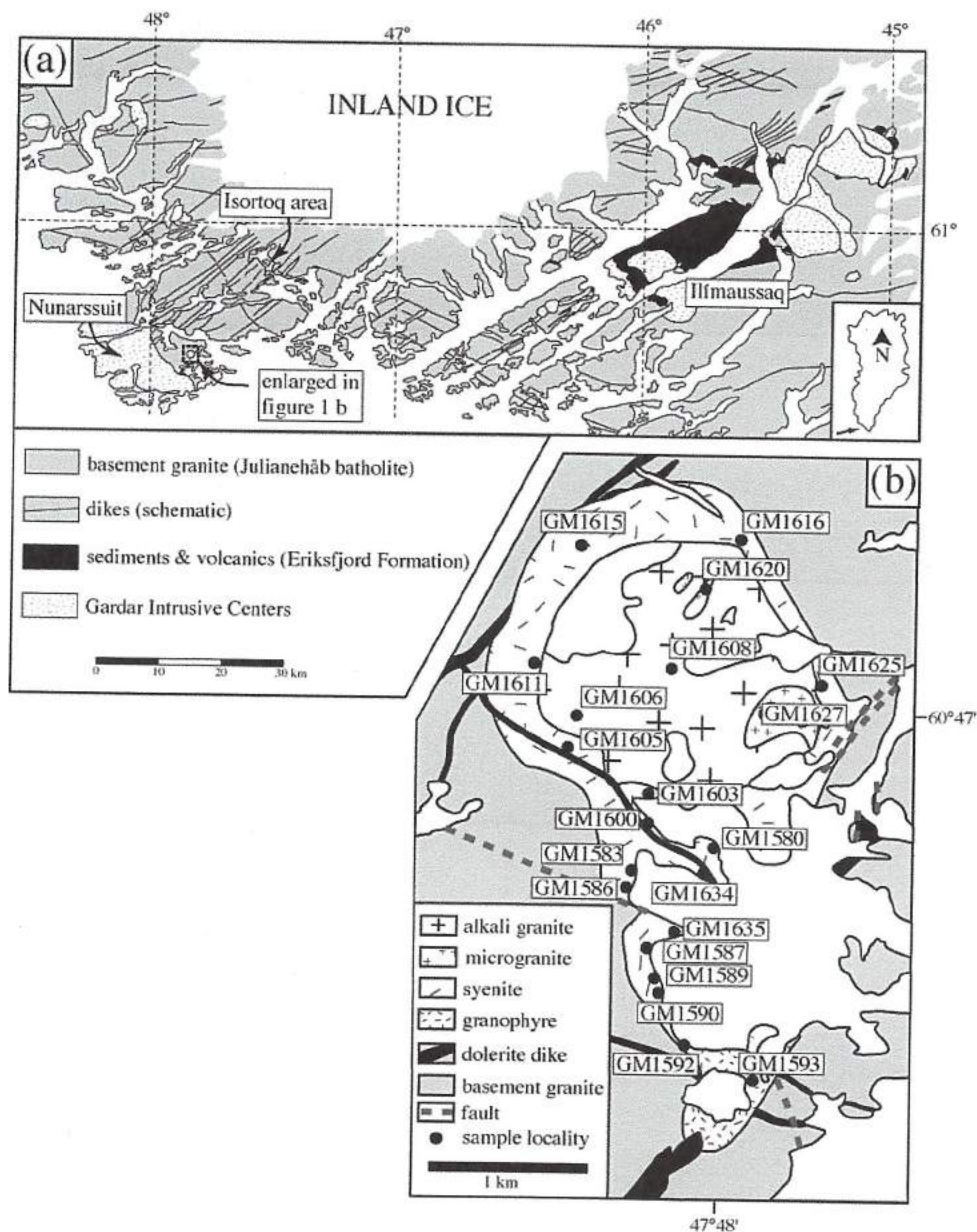
Fig. 1. (a) Sketch map of the alkaline Gardar Province, South Greenland [modified after Escher & Watt (1976)]. The Puklen complex is situated in the western part of the province. Nunarssuit and Ilmaussaq are other alkaline complexes referred to in the text. (b) Enlarged detail of (a). Generalized geological map of the Puklen complex, South Greenland [based on Parsons (1972)]. ●, sample localities.
