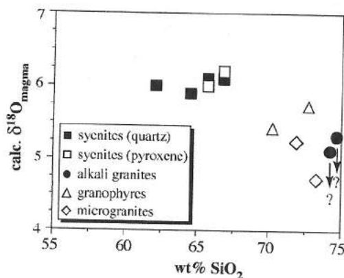
Fig. 16. Calculated oxygen isotopic compositions for the Puklen melts after the methods of Kalamirides (1986), Taylor & Sheppard (1986) and Harris (1995). The homogeneous values for the syenitic parental melt are in contrast to significantly lower and rather inhomogeneous values for the other rock types. The calculated \delta^{18}\text{O}_{\text{melt}} values for coarse alkali granites are maximum estimates. (See text for further explanation.)
