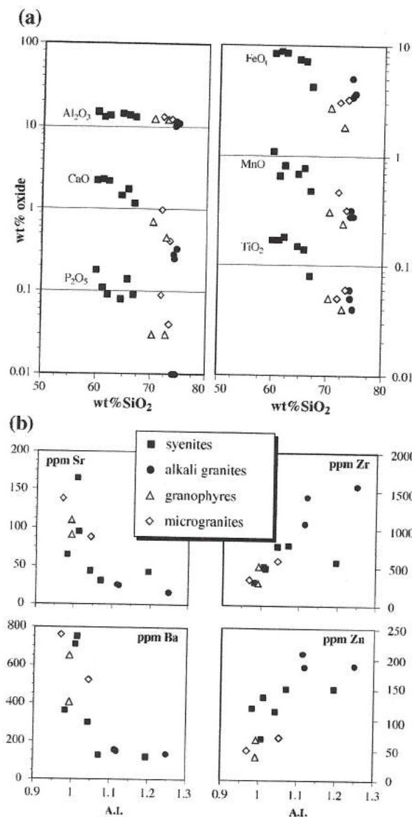
Fig. 8. (a) Major element variation diagrams for the Puklen rocks. SiO 2 is used as x-axis. (Note the logarithmic scale of the y-axis.) (b) Minor element variation diagrams for the Puklen rocks, with A.I. [algaipic index; molar ratio of (Na 2 O + K 2 O)/Al 2 O 3 ] as x-axis. The syenite sample with the exceptionally high A.I. of 1.2 is sample GM1611, which is a totally metasomatized sample.
