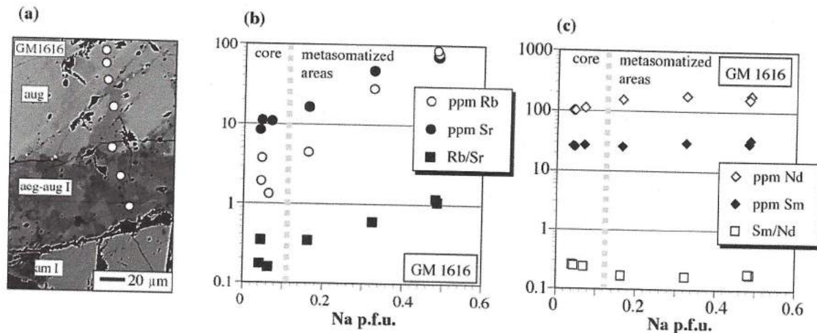
Fig. 7. Trace element data for augite of sample GM1616, which is metasomatized along cracks and grain boundaries by a late-stage fluid phase (compare Fig. 3a). (a) BSE image with data points indicated as white circles. (b) Rb and Sr concentrations plotted against Na p.f.u., which is used as an indicator for increasing metasomatism. The dashed grey line separates measurements in virtually unaffected core regions (left) from metasomatized areas (right) of the same grain. (c) Sm and Nd data for the same data points. Note the logarithmic scale of the y-axis.
