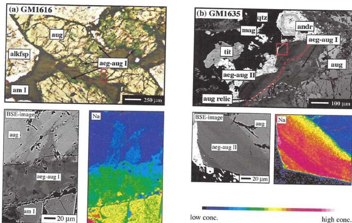
Fig. 3. (a) Top: photomicrograph (plane-polarized light) of augite, which is metasomatized along cracks and grain boundaries by a fluid phase (sample GM1616). Bottom: BSE image (left) and element map for Na (right) of a typical Na-enriched area. (b) Top: BSE image of aegirine-augite II rim around primary augite (sample GM1635). Secondary phases include hydroandradite, titanite, Ti-free magnetite and quartz. The dashed red line represents the assumed former grain boundary of primary augite. The dashed white line outlines a relic of primary augite. Bottom: BSE image (left) and element maps for Na (right) of an aegirine-augite II rim, which shows oscillatory zonation.
