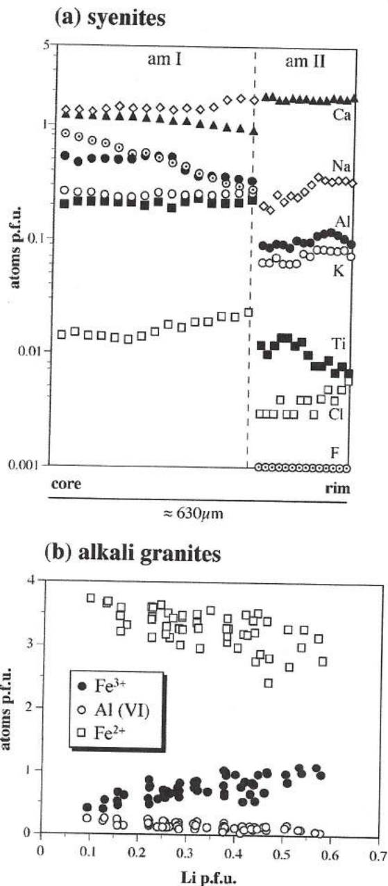
Fig. 6. Amphibole compositions. (a) Zoning profile starting in the core of an interstitial amphibole I through a rim of later amphibole II in syenite. (Note the logarithmic scale of the y-axis.) (b) Li vs \text{Fe}^{3+} , Al(VI) and \text{Fe}^{2+} for the Li-amphiboles in alkali granites. For amphibole I in the syenites and amphibole in the granites, calculated formulae are based on 16 cations and 23 oxygens, assuming a completely filled A site. Formulae for amphibole II in the syenites are calculated after the method of Schumacher, described by Leake et al. (1997).
