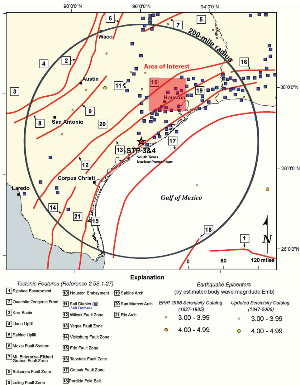
Figure 1: Principal Regional Faults in Texas Passing through the Houston, Texas Area and Environs See Figure 1A for Regional Geology and Growth Fault Distribution ( click here ). (Modified from Nuclear Regulatory Commission, [286].)
