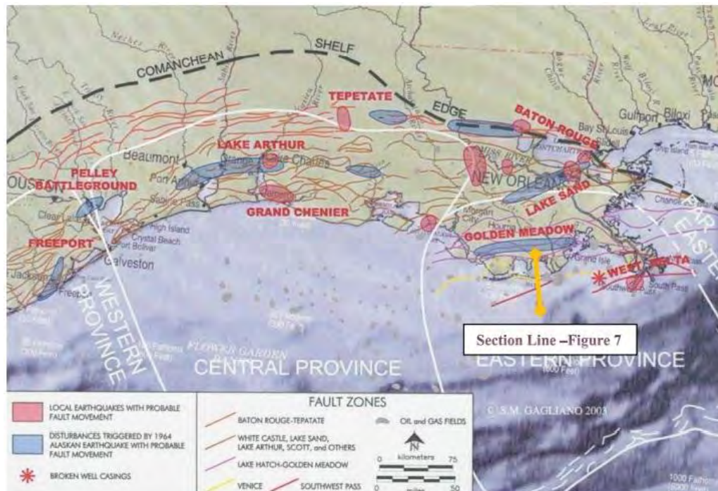
Figure 8: Plan View of Principal Growth Faults in Louisiana and Texas, and Areas Disturbed by 1964 Earthquake in Alaska. [40].
