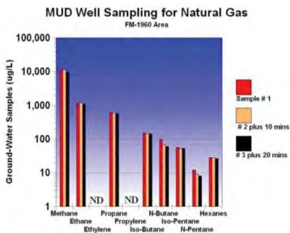
Figure 27: Head-Space Sampling of MUD Well. (From [10]).
