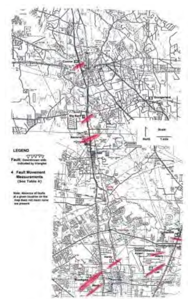
Figure 49: Principal Active Faults, North Harris, Conroe and Montgomery Counties, Texas (After [205]) (Click to Enlarge).
