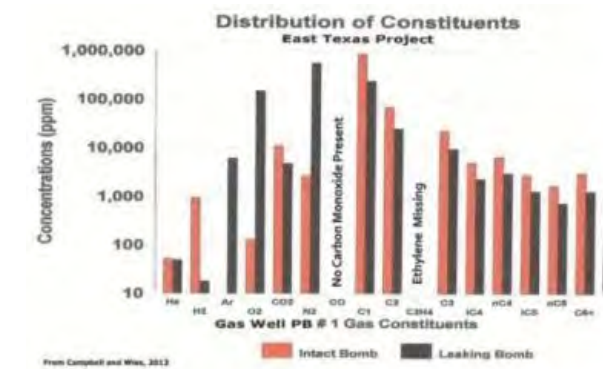
Figure 32: Sampling Results: Natural Gas Well. From [10]) ( Click to Enlarge )
