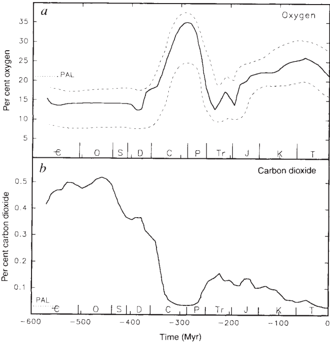
FIG. 1 a, Palaeoatmospheric oxygen concentration model 6 showing the estimate (solid line) and its range (dashed lines), based upon sensitivity analysis. Between the mid-to-late Devonian (380–360 Myr), oxygen increased from ~18 to 20%, and then rose sharply to ~35% by late Carboniferous (286 Myr). The present atmospheric level (PAL) of 21% is indicated. Oxygen steadily declined throughout the Permian (286–250 Myr) and dropped to about 15% by the end of the Palaeozoic (250 Myr). Model is based on the exchange rate of fixed carbon between the atmosphere, ocean and sediments 4,6,7 and on various assumptions 6,9,83 . b, Palaeozoic atmospheric carbon dioxide model 7–9 . This gas was present in relatively large amounts in the Ordovician–Silurian, fell precipitously during the Devonian–Carboniferous, and increased in the late Permian. The minimum value shown for the late Carboniferous and early Permian approximates PAL for carbon dioxide (about 0.036%; dotted line). Model is based on estimates of fixed carbon exchange and transfer processes within the inorganic, carbonate–silicate cycle 1,7,8 .
