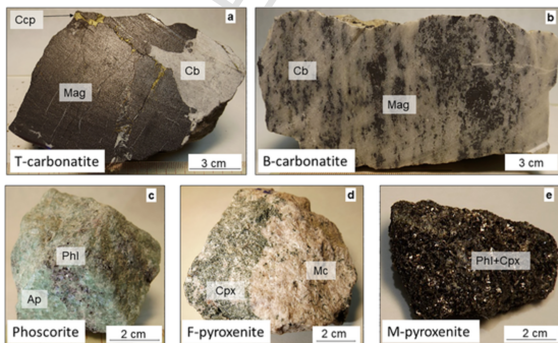
Fig. 2. Rocks fragment from the waste rock dumps of Phalaborwa Igneous Complex; (a) magnetite-rich section of T-carbonatite composed by magnetite (Mag), carbonates (Cb) and chalcopyrite (Ccp) filling fractures; (b) B-carbonatite formed of alternating band of carbonates (calcite and dolomite) and magnetite (Mag); (c) fluorapatite-rich phoscorite comprised of fluorapatite (Ap) associated with phlogopite (phl); (d) F-pyroxenite formed by microcline (Mc) and clinopyroxene (cpx); and (e) M-pyroxenite composed by phlogopite and clinopyroxene.
