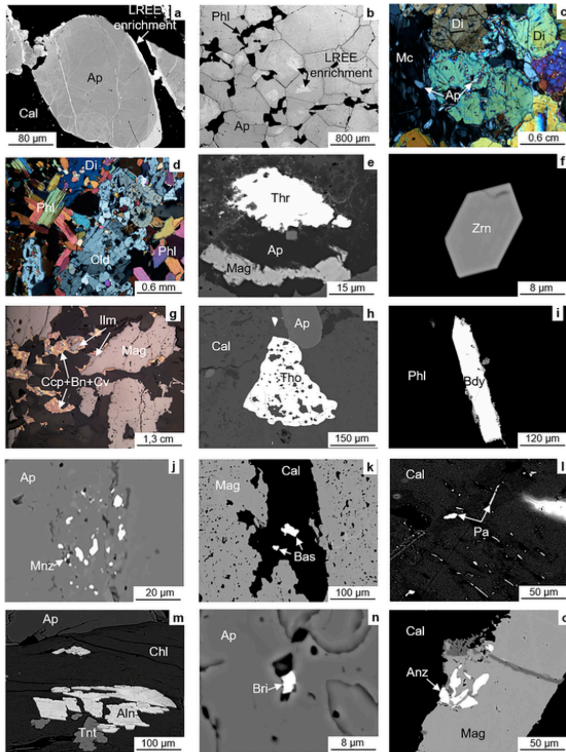
Fig. 3. Reflected light and backscattered electron (BSE) images of the waste rocks; a) LREE enrichment along grain boundaries of subhedral fluorapatite (Ap) included in calcite (Cal), from T-carbonatite; b) phlogopite (Phl) filling interstices in fluorapatite aggregate with LREE enrichment in the core grains, from Phoscorite; c) diopside (Di) aggregate with apatite inclusions and microcline (Mc) filling open spaces, from F-pyroxenite; d) phlogopite aggregate associated with chloritoid (Cl) and diopside, from M-pyroxenite; e) thorite (Thr) filling spaces in apatite and magnetite (Mag); f) euhedral zircon (Zrn) grain included in calcite, from F-Pyroxenite; g) chalcopyrite (Ccp), bornite (Bn) and covellite (Cv) filling open space in magnetite, ilmenite (Ilm) and calcite crystals, from T-carbonatite; h) thorianite (Tho) replacing calcite, from B-carbonatite; i) acicular baddeleyite (Bdy) included in phlogopite, from T-carbonatite; j) monazite (Mnz) inclusions in fluorapatite, from B-carbonatite; k) bastnäsite (Bas) grains in calcite, from T-carbonatite; l) parisite (Pa) crystals associated with calcite, from B-carbonatite; m) titanite (Tnt) and allanite (Aln) interbedded with chlorite (Chl), from F-pyroxenite; n) britholite (Bri) inclusions in fluorapatite, from B-carbonatite; o) anzaitite (Anz) included in magnetite, from F-pyroxenite.
