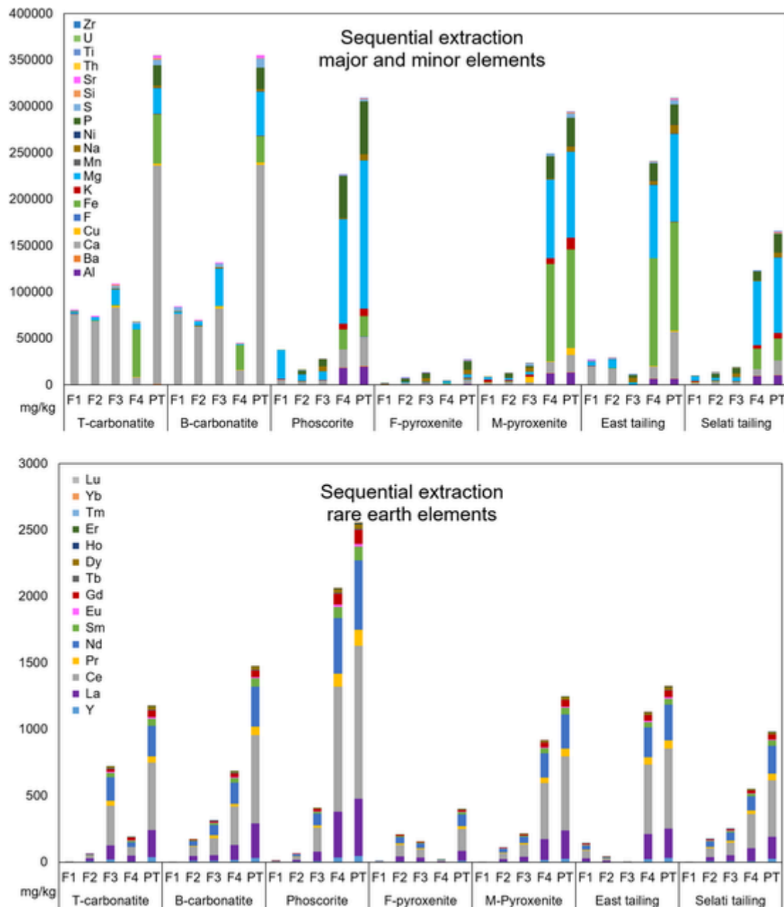
Fig. 7. Elemental distribution of PIC's main lithologies and tailings in each step of the sequential extractions (F1, F2 F3 and F4) and the pseudo-total concentration in the aqua regia digestion (PT). (For interpretation of the references to colour in this figure legend, the reader is referred to the web version of this article.)
