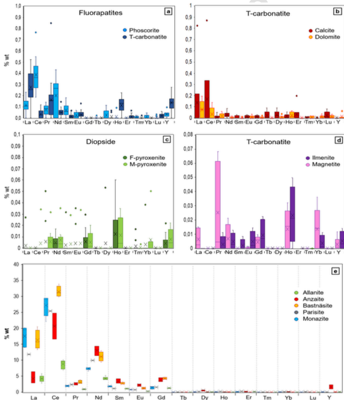
Fig. 4. Rare earth elements distribution in both REE-bearing minerals and REE-minerals in waste rock dumps based on electron microprobe analyses (EPMA) analyses; a) Fluorapatite from phoscorites and T-carbonatite; b) Calcite and dolomite from T-carbonatite; c) Diopside from F-pyroxenite and M-pyroxenite; d) Ilmenite and magnetite from T-carbonatite; and e) REE content in allanite, anzaitite, bastnäsitite and parisite included in T-carbonatite; and monazite from both T- and B-carbonatite rocks. Extended data included in Appendix 4 as oxide percentages.
