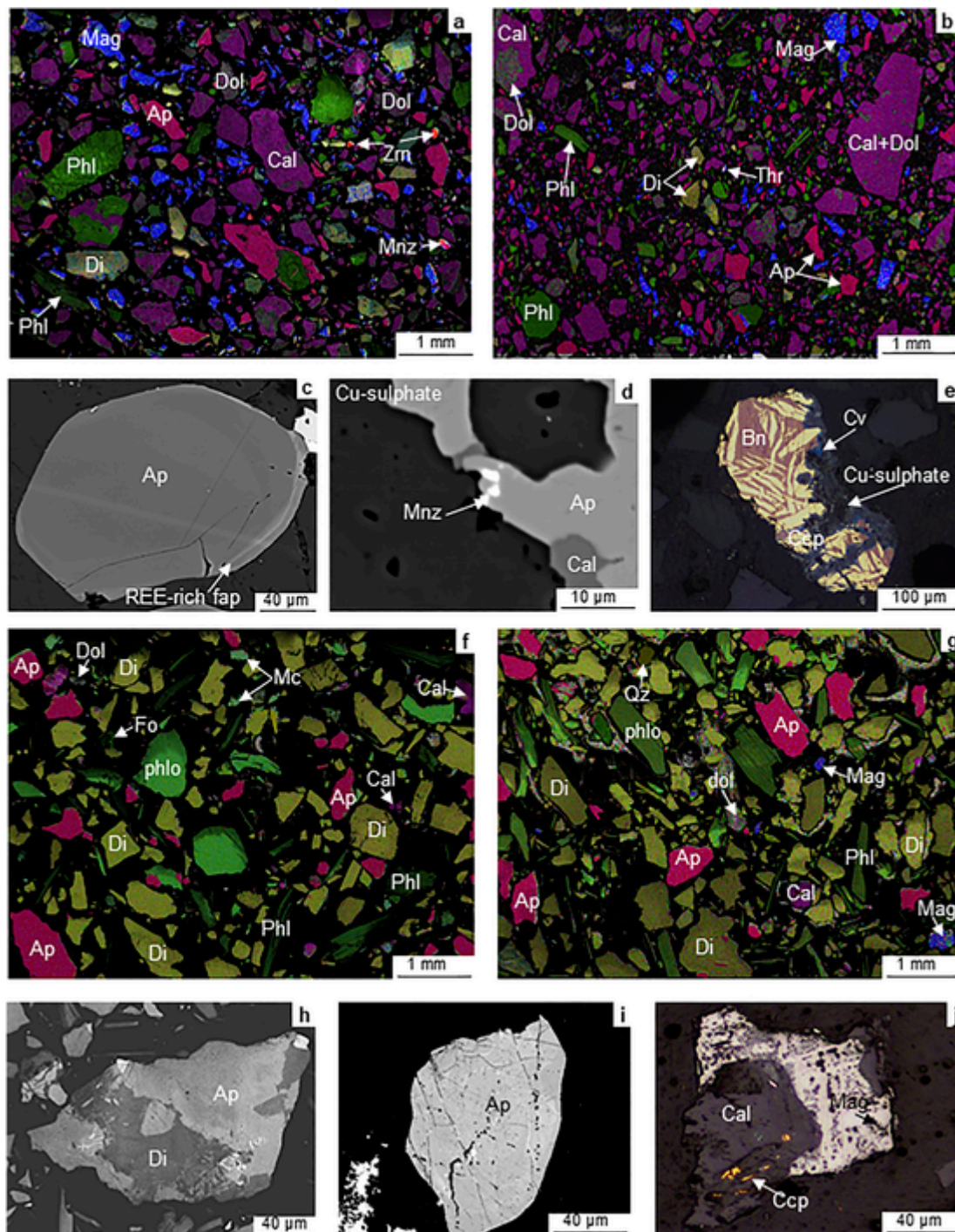
Fig. 5. False-colour compositional scanning electron microscope (SEM) maps, petrographic microscope and backscattered electron (BSE) images of tailings samples; (a) and (b) Compositional SEM maps from East tailing showing the major mineralogy, including calcite (Cal), dolomite (Dol), fluorapatite (Ap), diopside (Di), phlogopite (Phl), magnetite (Mag), zircon (Zrn) and monazite (Mnz); (c) fluorapatite showing a REE enrichment along grain boundaries; (d) monazite inclusions in fluorapatite; (e) mixed-fragment formed by chalcopyrite (Ccp), bornite (Bn), covellite (Cv) and newly-formed Cu-sulphate; (f) and (g) compositional SEM maps from Selati tailing showing the major mineralogy, such as phlogopite, diopside, fluorapatite, calcite, microcline (Mc), quartz (Qz), dolomite, magnetite and forsterite (Fo); (h) mixed fragment composed by diopside and fluorapatite; (i) subhedral fluorapatite included in calcite; (j) chalcopyrite and magnetite filling open spaces in calcite.
