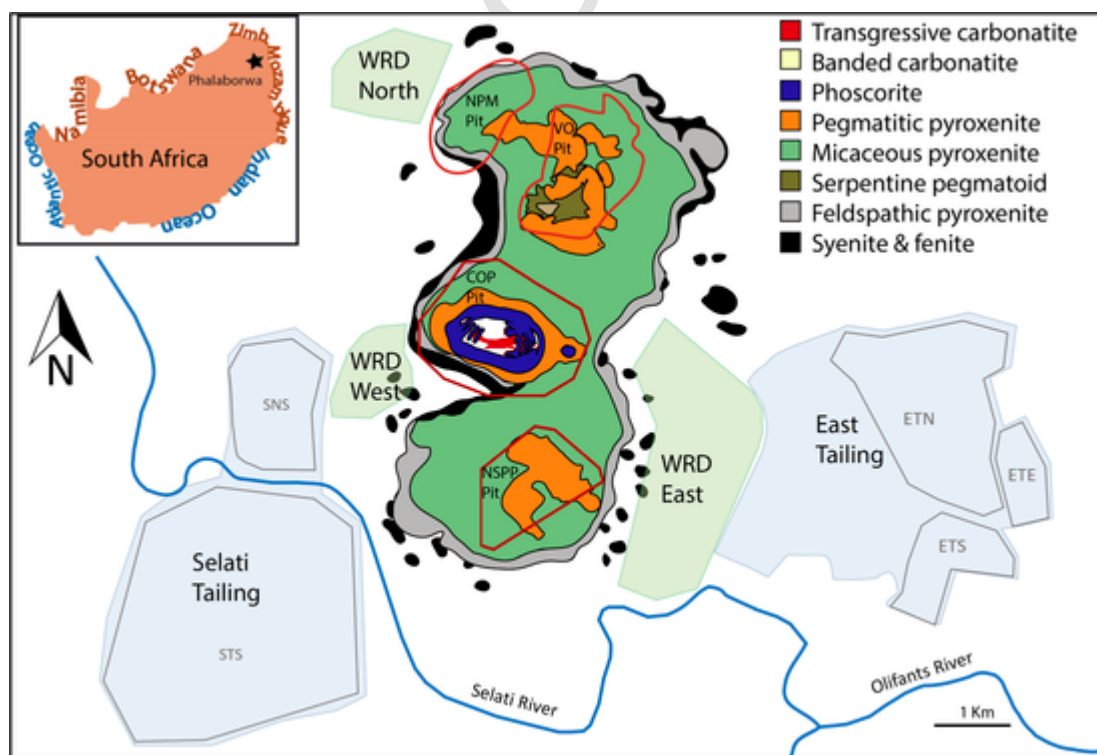
Fig. 1. Simplified geological map of Phalaborwa Igneous Complex (modified from Giebel et al., 2019) with the industrial structures, including: in red the Cu open pit (COP), the North Pyroxenite Mine (NPM) pit, the New South Pyroxenite Pit (NSPP) and Vermiculite Open (VO) Pit; Blue shadows represent the East and Selati tailing dams with each tailing sector marked in grey; and shaded in green are represented the waste rock dumps (WRDs). (For interpretation of the references to colour in this figure legend, the reader is referred to the web version of this article.)
