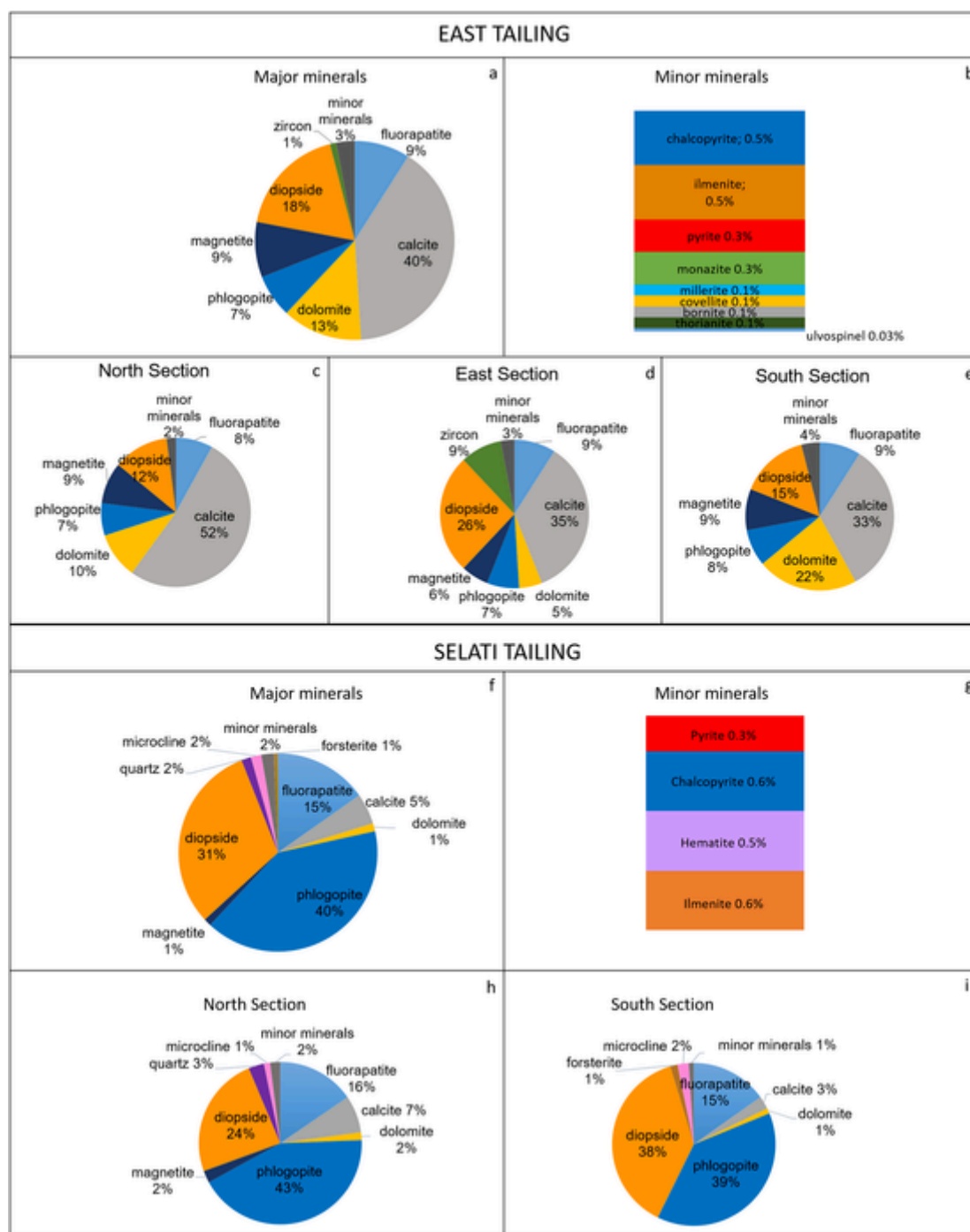
Fig. 6. Mineralogical semi-quantification based on image analysis of scanning electron microscope (SEM) compositional maps of the East tailing: (a) major minerals, (b) minor minerals, (c) major minerals of north section, (d) of east section, (e) of south section; and the Selati tailing (f) major minerals, (g) minor minerals, (h) major minerals of north section and (i) south section.
