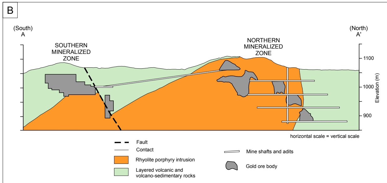
Figure 10Q. The Mahd adh Dhahab gold deposit, Saudi Arabia (modified from Doebrich, 1999). A. Generalized geologic map showing geologic units, faults, and the distribution of quartz veins. B. North-south cross section A-A' through the Northern and Southern Mineralized Zones.
