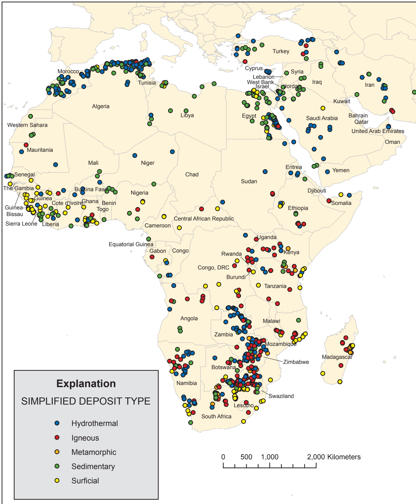
Figure 9A. Map showing distribution of principal nonfuel mineral deposits in Africa and the Middle East by simplified deposit type. There is a tendency for surficial laterite deposits to form in tropical settings near the equator; surficial placer deposits form in fluvial, lacustrine, and coastal marine environment. Hydrothermal deposits tend to form in mountain ranges and in basins affected by orogenic activity and igneous deposits to be localized in island arcs, continental margin arcs, and to a lesser extent in stable shields.
