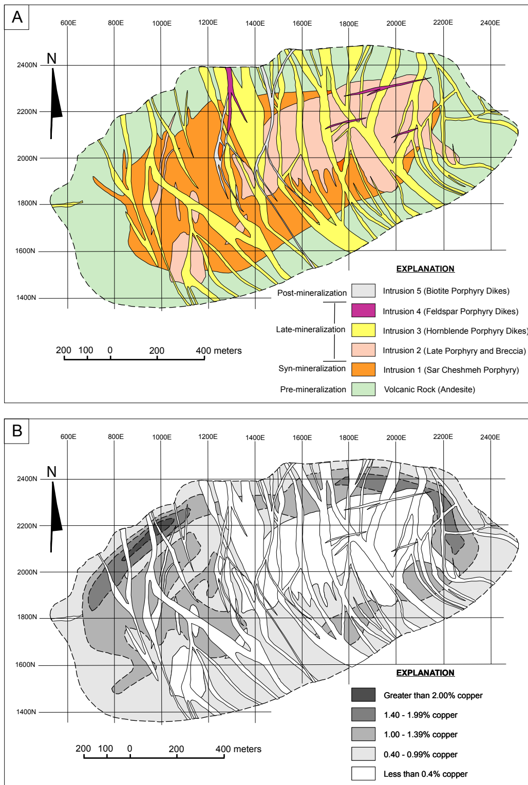
Figure 10P. The Sar Cheshmeh copper deposit, Iran (modified from Waterman and Hamilton, 1975). A. Distribution of rock types within the zone of greater than 0.4 percent copper, at the 2,400-meter elevation level. B. Distribution of copper grades at the 2,400-meter elevation level.
