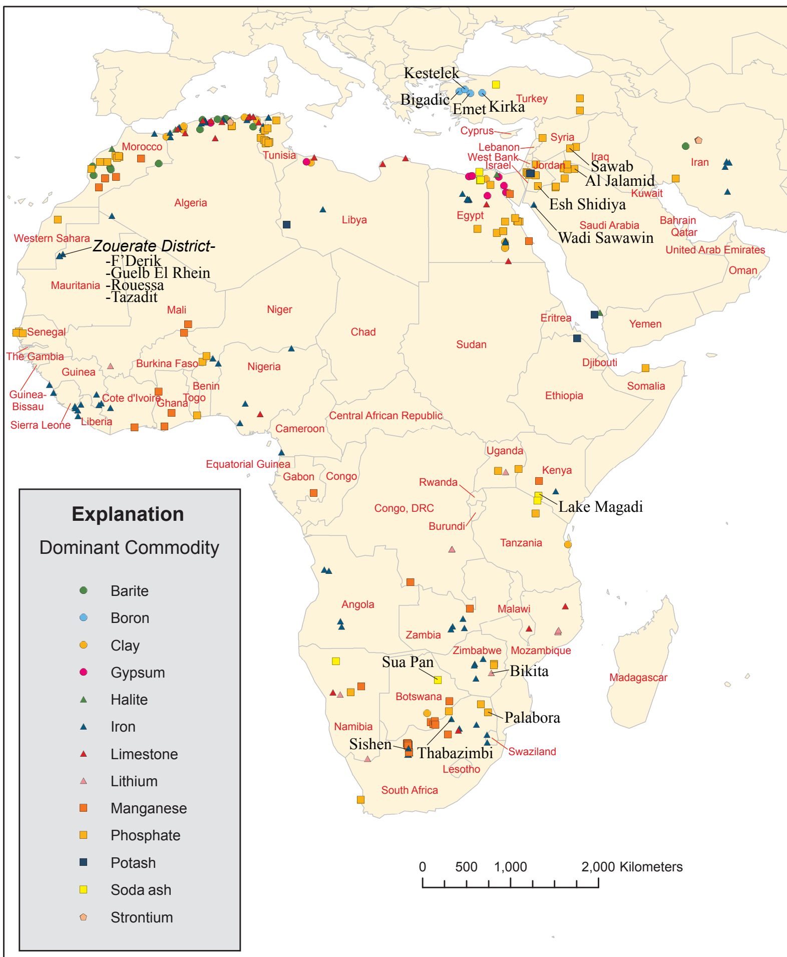
Figure 9D. Map showing location of major deposits of strontium, sodium carbonate, potash, phosphate, managanese, lithium, limestone, clay (bentonite and kaolin), iron, halite (salt), gypsum, boron, and barite.
