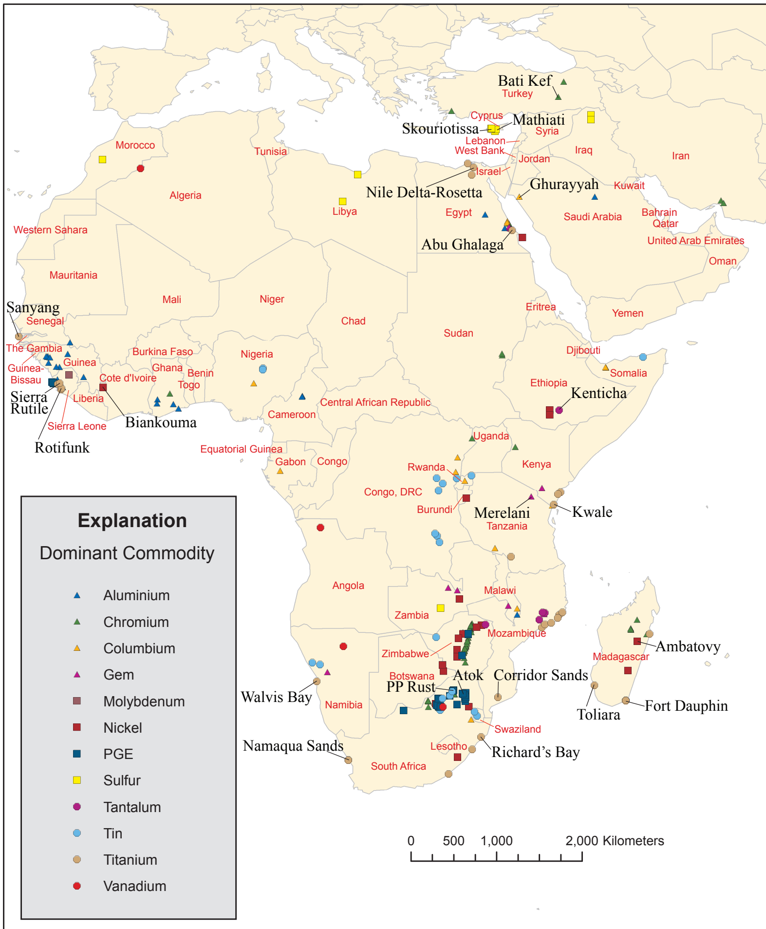
Figure 9E. Map showing location of major deposits of titanium, tin, tantalum, vanadium, sulfur, chromium, platinum-group elements (PGE), nickel, molybdenum, gemstones, columbium, and aluminum.
