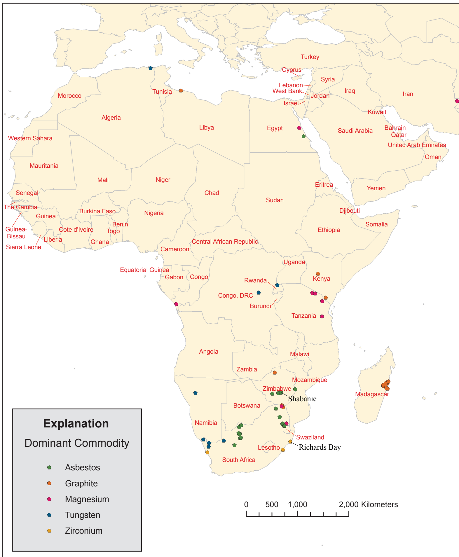
Figure 9F. Map showing location of major deposits of tungsten, magnesium, graphite, zirconium, and asbestos.
