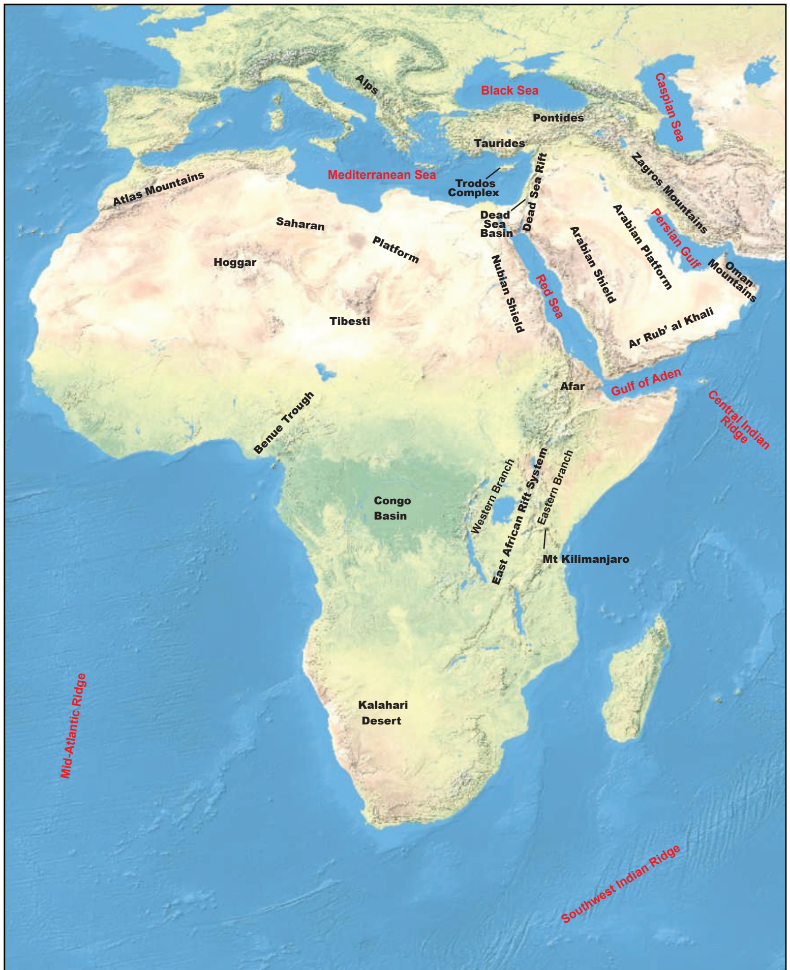
Figure 2. Digital elevation image of Africa, the Middle East, and the surrounding ocean basins. Major aspects of the geology of the world are evident in the differences in elevation (topography). Examples include folded mountain ranges (orogens) such as the Atlas Mountains, volcanic mountain ranges that encircle the globe beneath the sea (mid-ocean ridges), linear depressions formed where continental crust is being stretched (East African rift system), and topographic highs formed where geologically old, stable rocks that are the nuclei of continents (shields) are present (Arabian shield).
