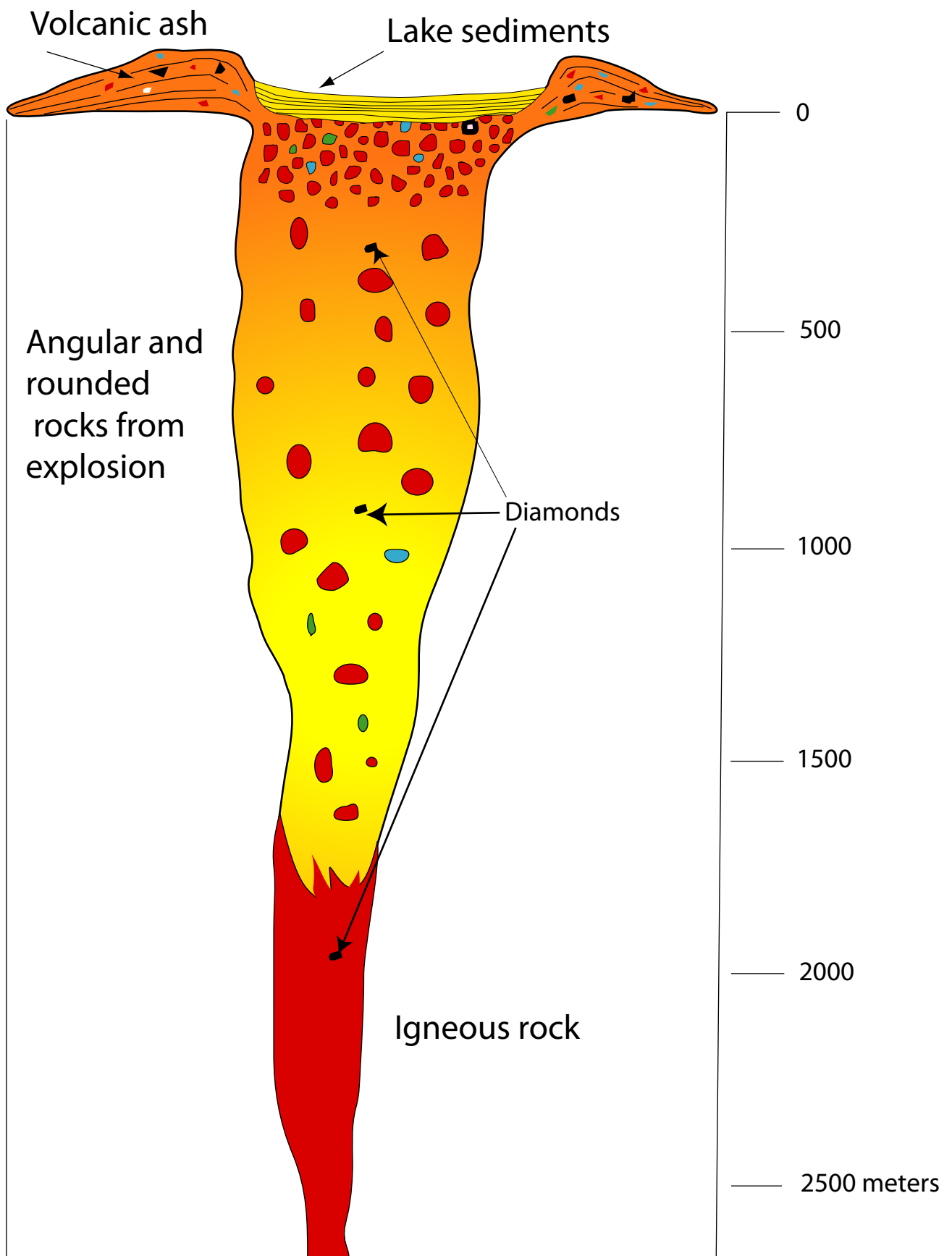
Figure 10N. Diagrammatic section of a diamond kimberlite pipe. These igneous intrusions are pipe-like bodies that form by explosive processes and consist of a distinctive type of dark rock called kimberlite. The magma that forms kimberlites originates in the Earth's mantle where pressures and temperatures are high enough to form diamonds. Adopted from Cunningham and others (this volume).
