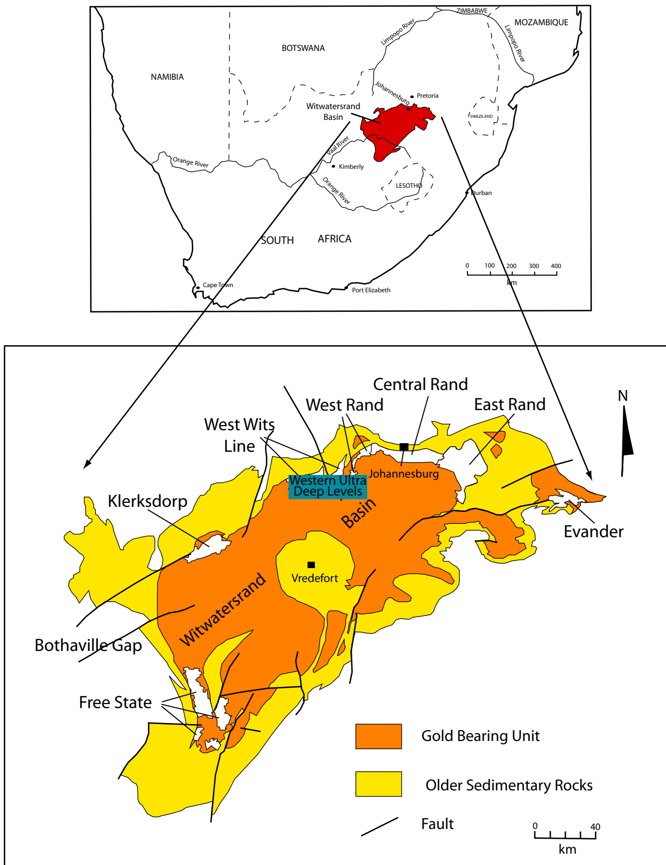
Figure 10J. Location map of the Witwatersrand Basin and its major goldfields. Modified from Robb and Robb (1998).
