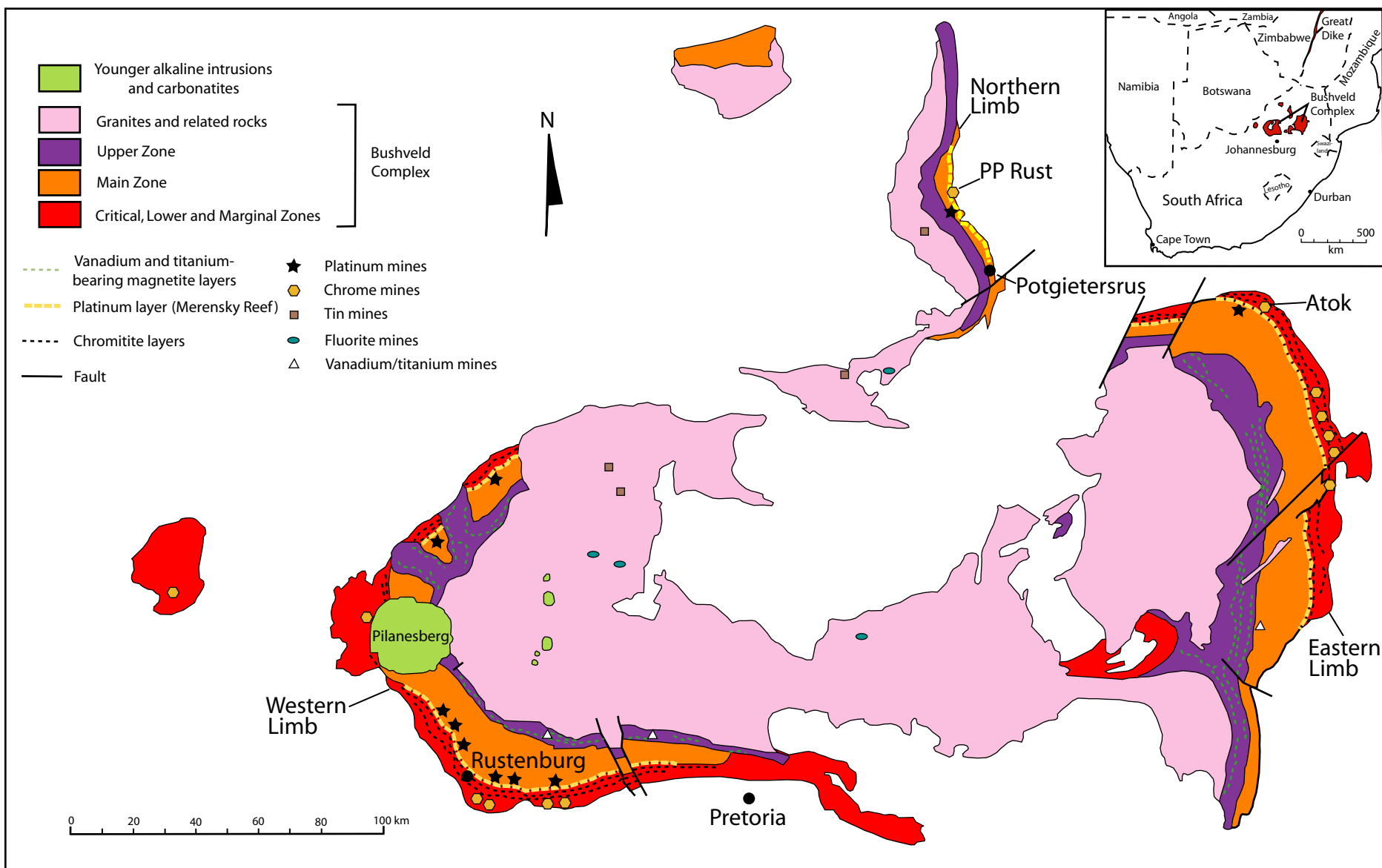
Figure 10H. Simplified geologic map of the Bushveld Igneous Complex, showing locations of some of the more important chromium and PGM mines. Modified from Viljoen and Schurmann (1998).
