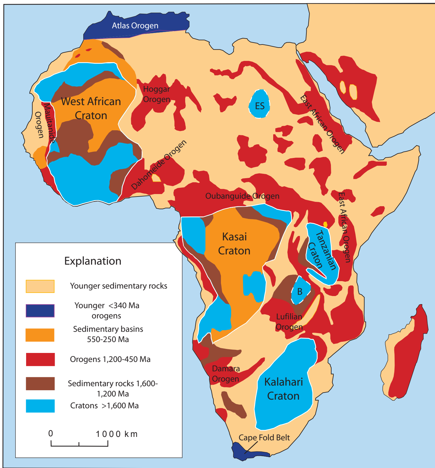
Figure 7A. Map showing selected geologic and tectonic features of Africa. The small cratonic nuclei of the Bangweulu craton is depicted with a "B" and the East Saharan craton with "ES". Modified from Dallmeyer and Lecorche (1991).
