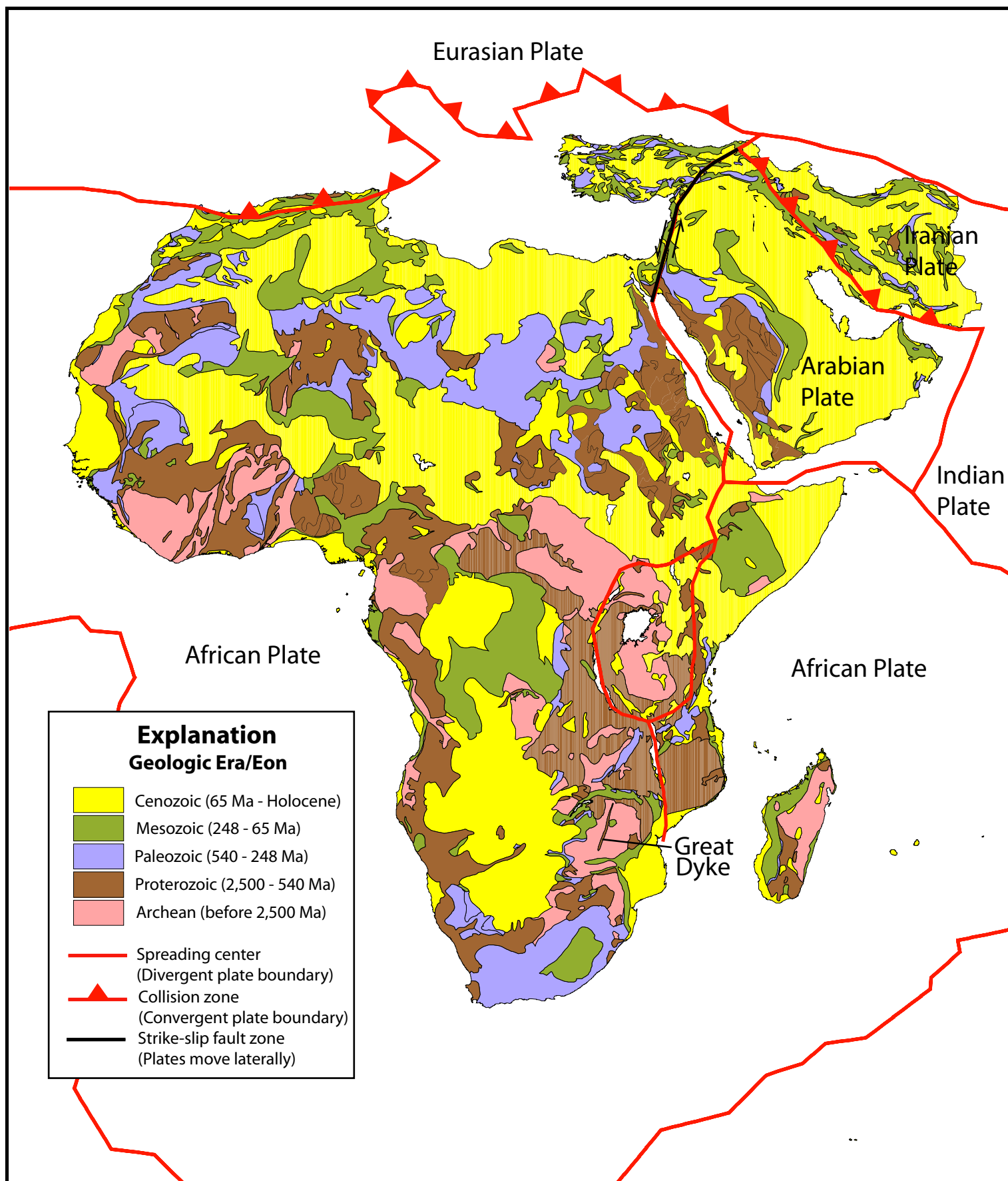
Figure 6. Geologic map of Africa and the Middle East showing the ages of principal rock units and the location of tectonic plate and plate boundaries. Modified from Kirkham and others (1995).
