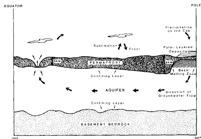
Fig. 4. Generalized model of the Martian hydrologic cycle.
