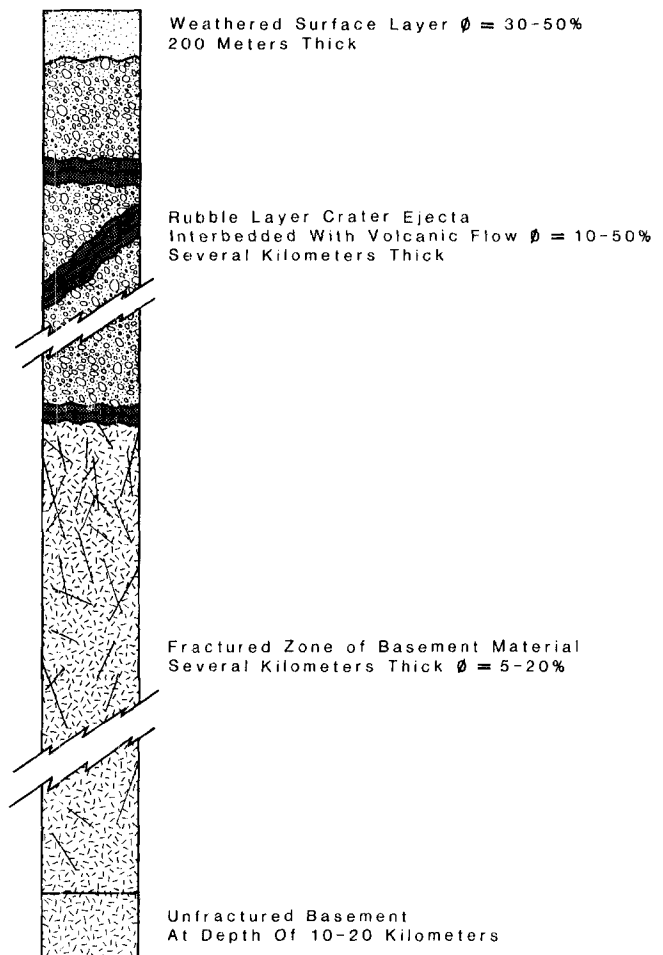
GENERALIZED STRATIGRAPHIC COLUMN OF MARS
