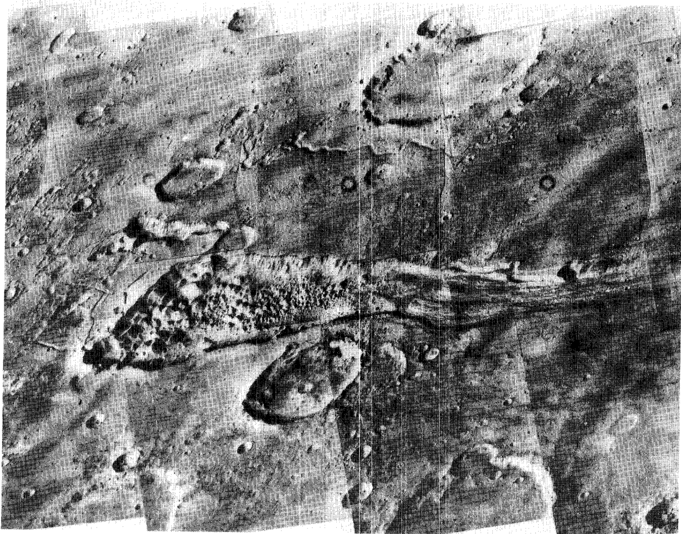
Fig. 2. Martian outflow channel near the Simund Vallis. NASA, Viking 1, P-16983. Scale is 1.5 cm = 20 km.
