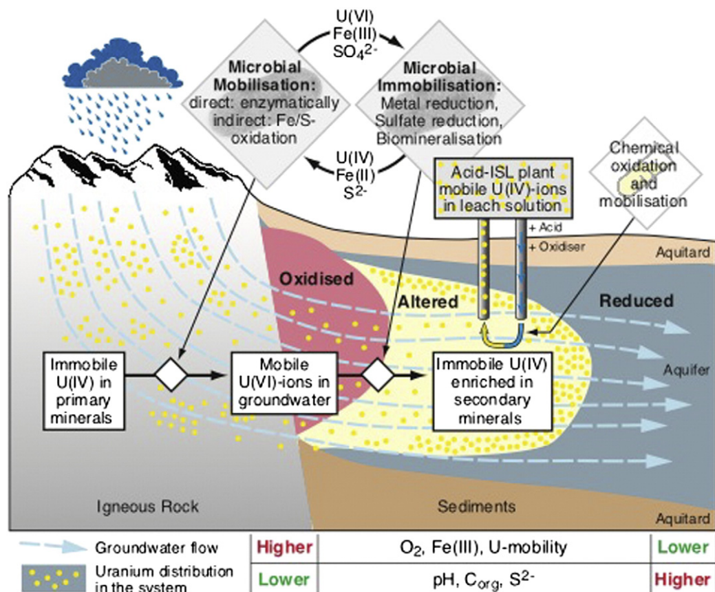
Fig. 5. Model of uranium roll-front deposit.
