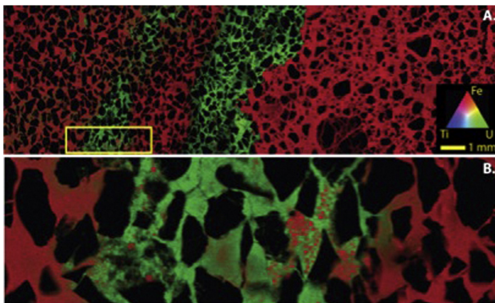
Fig. 4. Synchrotron X-ray fluorescence map of the distribution of U, Fe and Ti in a sandstone-hosted sedimentary ore from the Frome Embayment, South Australia. A. Full image, covering a 2 \times 0.6 \text{ cm}^2 area at 2 \mu\text{m} resolution. B. Detail of a U-rich band. The red spheres correspond to biogenic pyrite. The images are modified from (Zammit et al., 2013); they were obtained at the XFM beamline at the Australian Synchrotron (Paterson et al., 2011) using the 384-element Maia detector (Ryan et al., 2010; Etschmann et al., 2010). The X-ray images were processed and quantified using the GeoPIXE software (Ryan et al., 2010).
