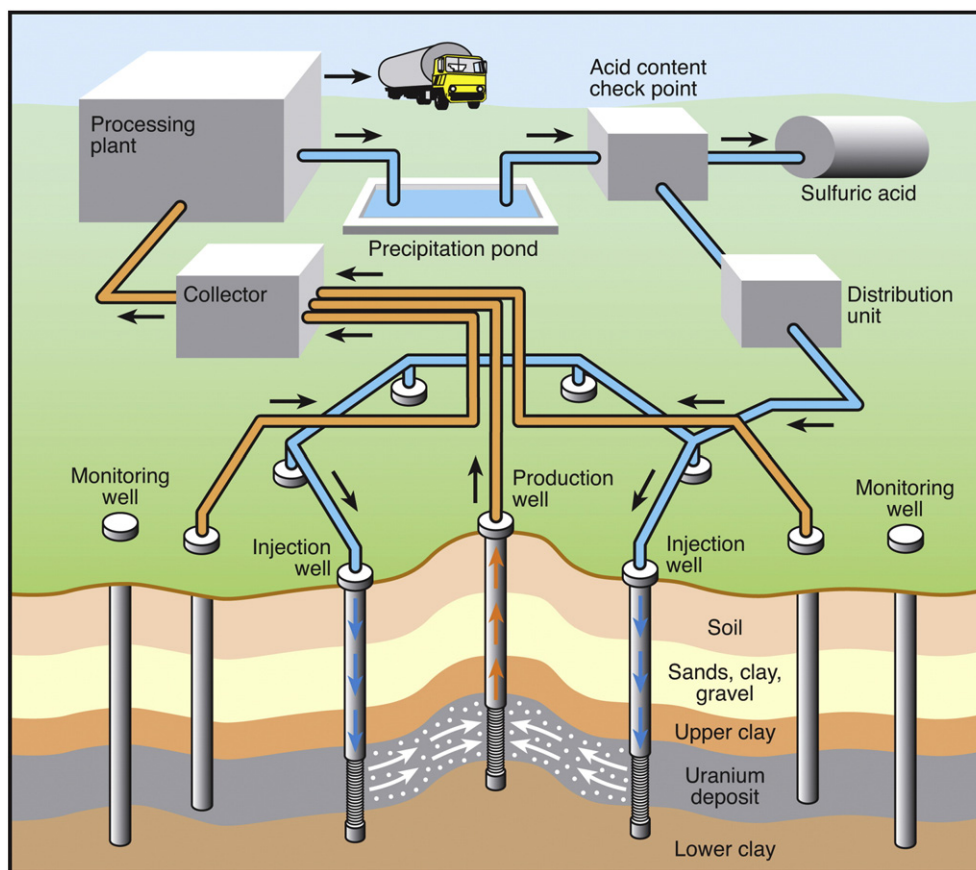
Fig. 3. In situ leaching operation. Adapted from Pannier (2009).
