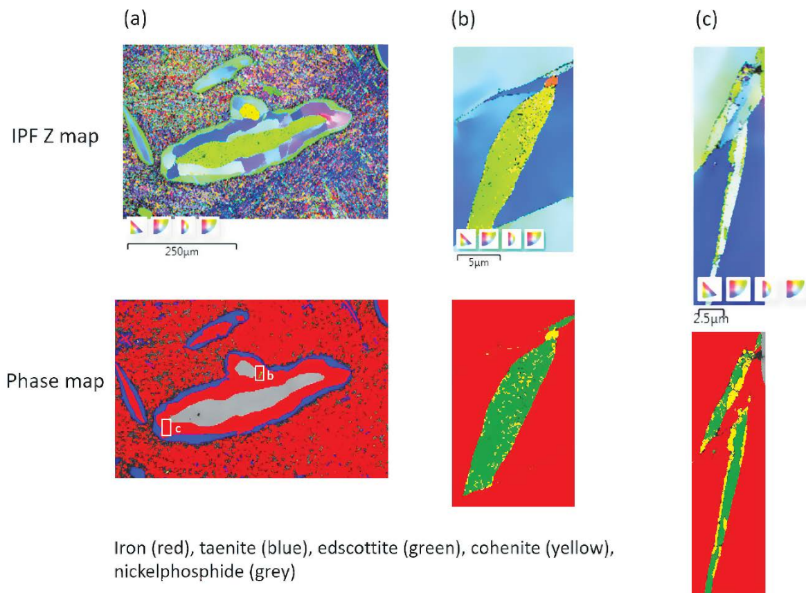
FIGURE 3. EBSD mapping. (a) The area corresponds roughly to Figure 1a. Two rectangles in its phase map outline regions in b and c . (b) A region corresponding roughly to Figure 1d and (c) another region showing cohenite along with edscottite. Top row: inverse pole figure (IPF) Z orientation maps; bottom row: phase maps. (Color online.)
