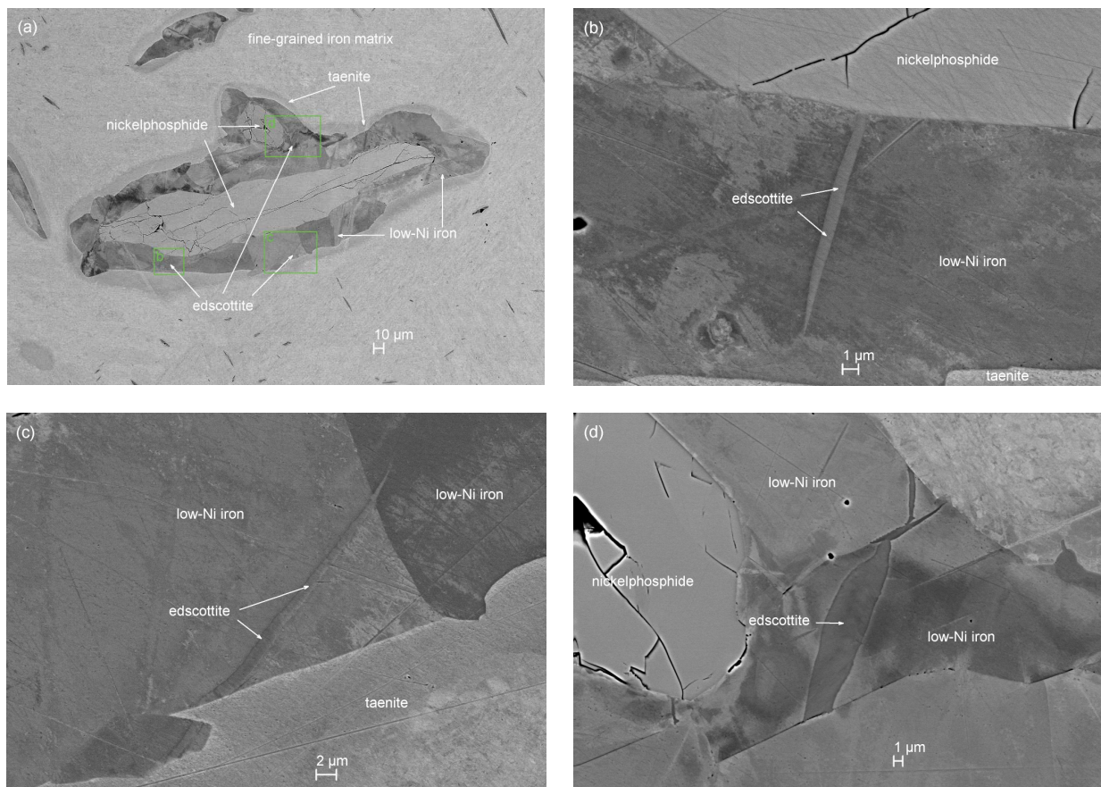
FIGURE 1. SEM BSE images showing edscottite with taenite, low-Ni iron, and nickelphosphide in the polished Wedderburn section UCLA 143. (a) Overview. (b, c, and d) Enlarged BSE images of rectangular regions outlined in panel a. (Color online.)
