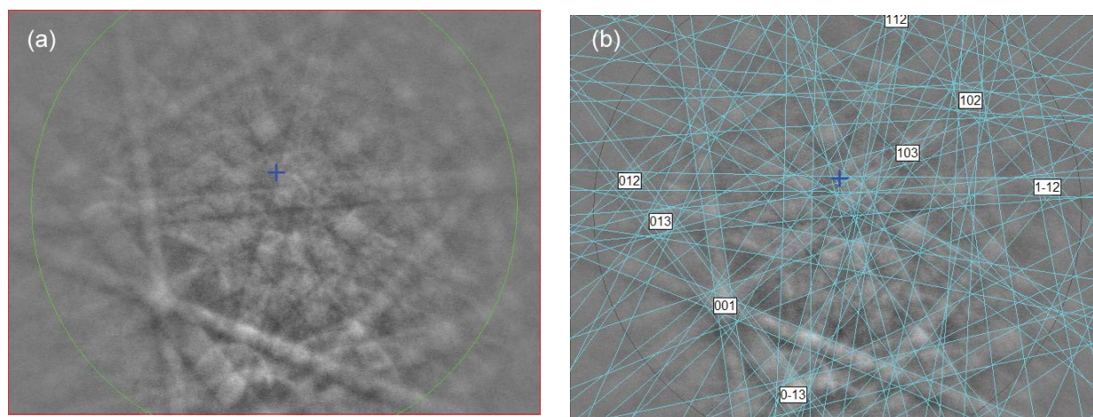
FIGURE 2. (a) EBSD pattern of one edscottite crystal in Figure 1, and (b) the pattern indexed with the \text{C2}/c \text{Fe}_3\text{C}_2 structure. (Color online.)
