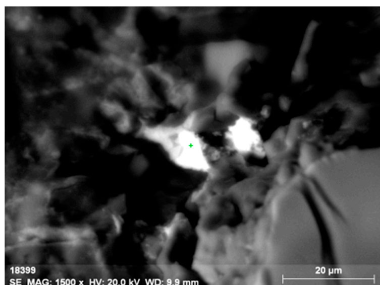
Figure 6. Microinclusion of uranothorianite (up to 1.9% of uranium) in orthite.
