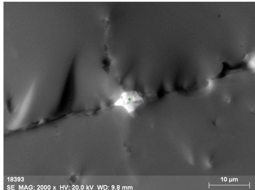
Figure 4. Micromineral phase of thorianite ( \text{ThO}_2 ) intersecting orthite.
