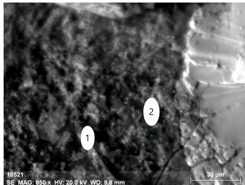
Figure 10. Mineral aggregate comprising yttrium-containing orthite with (1) the low content of REEs (dark grey) and (2) the thorianite aggregate (grey).
