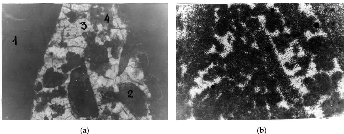
Figure 15. Distribution of uranium in the quartz-fluorite-orthite ore: (a) polished section, where nicols are parallel, 1, 2—orthite, 3—quartz, 4—fluorite; (b) fission radiography, dark areas correspond to microinclusions of uranium minerals.
