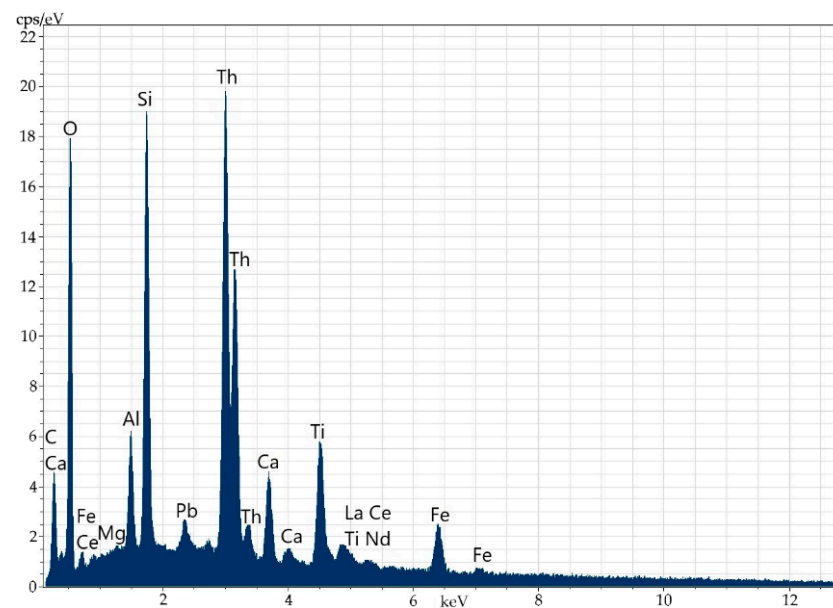
Figure 5. Energy-dispersive spectrum of the thorianite micromineral.
