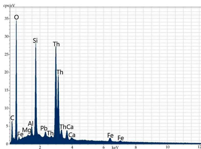
Figure 14. Energy-dispersive spectrum of the mineral phase of thorianite shown as a streak in orthite.
