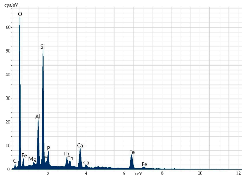
Figure 11. Energy-dispersive spectrum of orthite at point 1.
