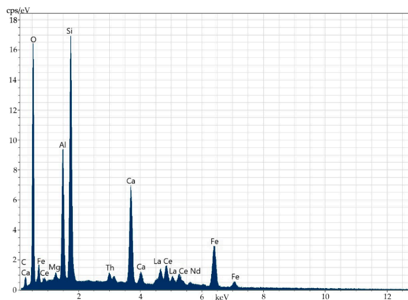
Figure 3. Energy-dispersive spectrum of the elements in the entire surface of the specimen.
