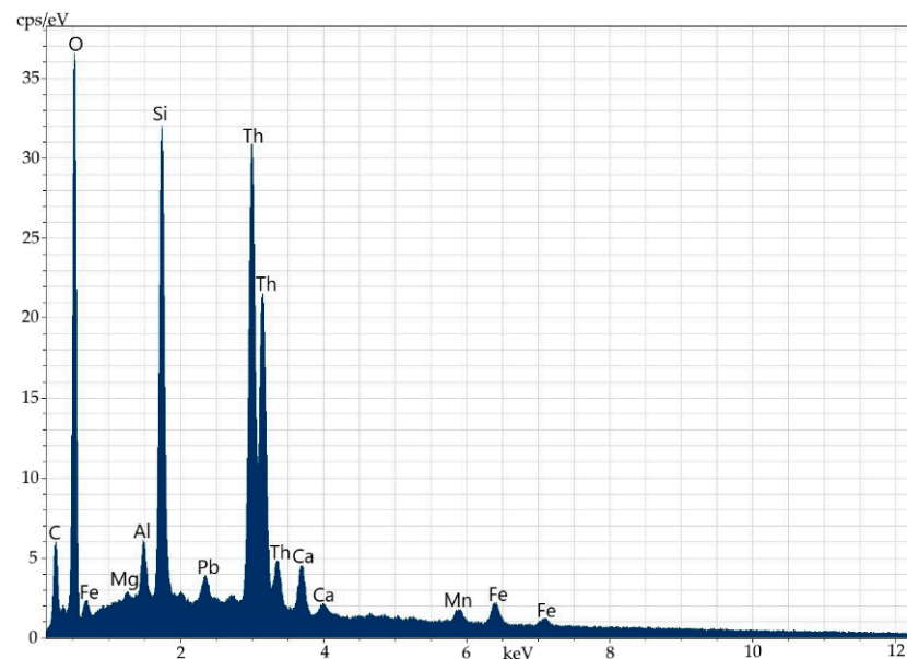
Figure 12. Energy-dispersive spectrum of thorium at point 2.
