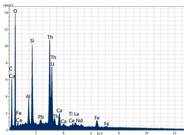
Figure 7. Energy-dispersive spectrum of the uranothorianite microinclusion in orthite.
