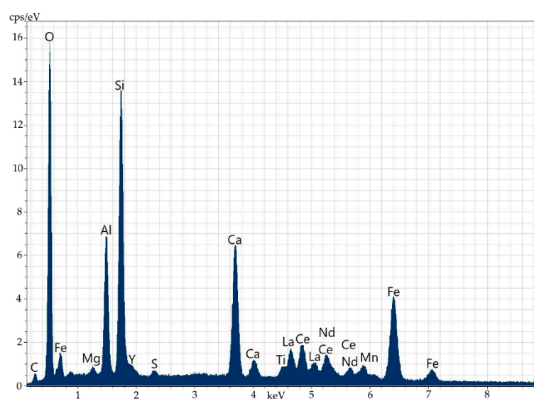
Figure 9. Energy-dispersive spectrum of thorium-less yttrium-containing orthite with REEs.
