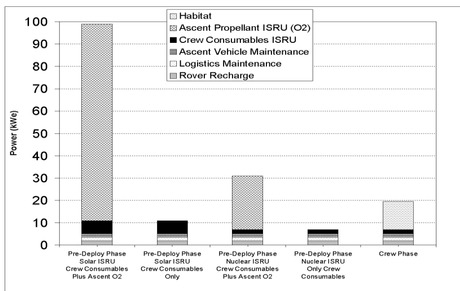
Figure 3-4: Quantitative Power Requirements
