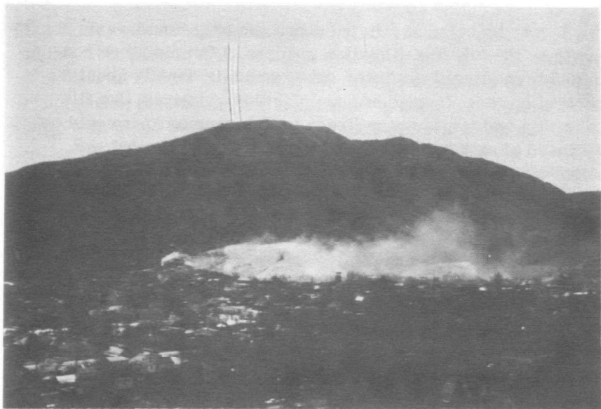
The light-colored tailings pile dominates this scene. Wind-blown particles of waste ore solids may be scattered over a wide area.
