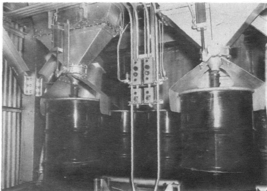
The filtered yellowcake is dried and packaged for shipment in 55-gallon drums. (Photograph courtesy of The Anaconda Company)
