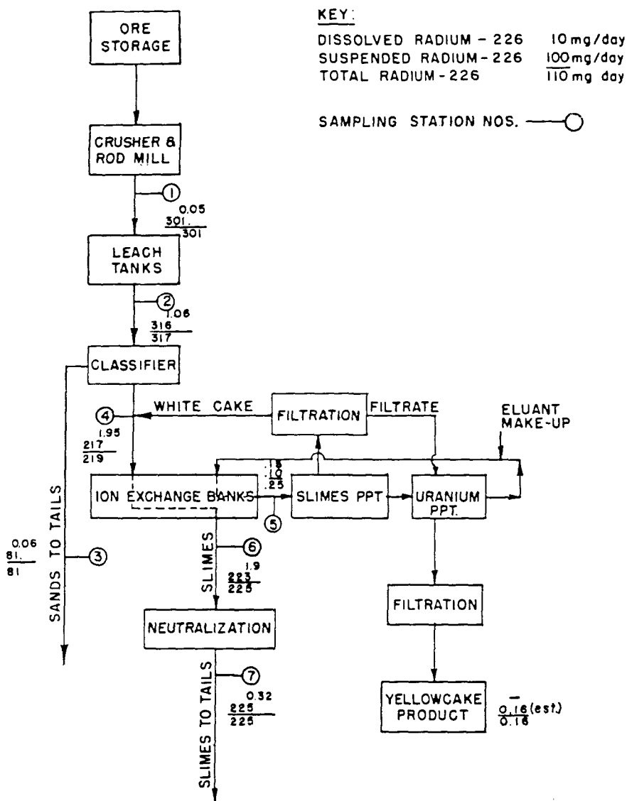
Figure 9. Schematic flow diagram, radium-226 balance - acid leach-RIP mill
