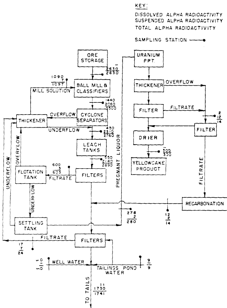
Figure 11. Schematic flow diagram, gross alpha radioactivity - alkaline leach mill.
