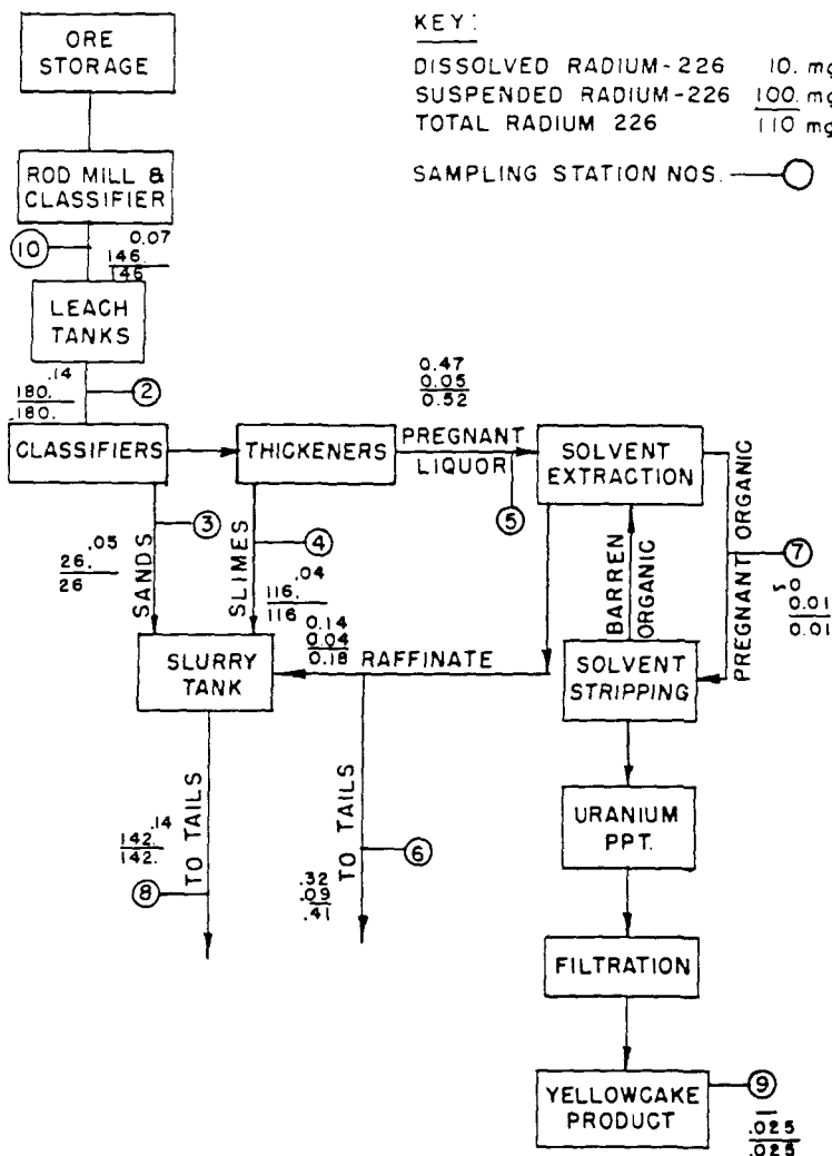
Figure 10. Schematic flow diagram, radium-226 balance - acid leach-SX mill.
