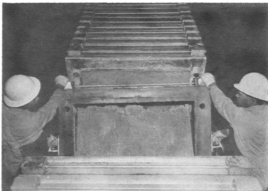
The dissolved uranium is precipitated and filtered. A plate and frame filter press is shown. (Photograph courtesy of The Anaconda Co.)
