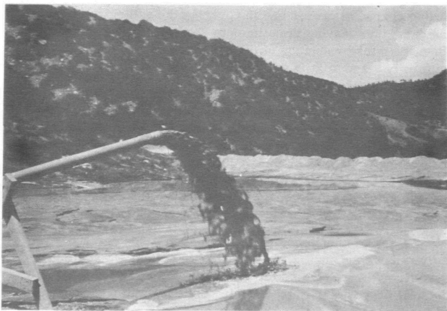
The waste ore slurry is pumped to a tailings pond where the solids are separated and retained.
