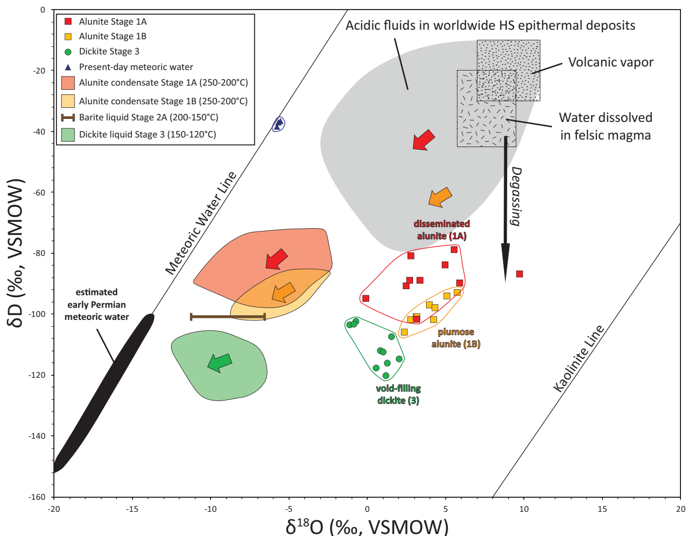
Fig. 11. Plot of \delta^{18}\text{O} versus \delta\text{D} values of stage 1A and stage 1B alunite ( \delta^{18}\text{O}_{\text{SO}_4} plotted) and stage 3 dickite from Mt. Carlton. The calculated compositions of hydrothermal condensates in equilibrium with stage 1A and stage 1B alunite are plotted together with compositions of magmatic vapor discharged from high-temperature volcanic fumaroles (Giggenbach, 1992), water dissolved in felsic magma (Taylor, 1992), estimated early Permian meteoric water (latitude \sim 36^\circ\text{S} ; Scotese, 2001; this study), present-day Mt. Carlton meteoric water (latitude \sim 20^\circ\text{S} ; \delta^{18}\text{O} = -5.8 to -5.5\text{‰} , \delta\text{D} = -39 to -37\text{‰} ; F. Sahlström, unpub. data, 2015), and acidic fluids related to advanced argillic alteration of worldwide high-sulfidation (HS) epithermal deposits (Arribas, 1995a, and references therein). The trends defined by stage 1A and stage 1B alunite-forming fluids indicate condensation of magmatic vapor by local meteoric water ( \sim 50 – 60\% meteoric component). The stage 2A barite ( \delta^{18}\text{O} values only) and stage 3 dickite liquid compositions are also plotted, indicating an increasing meteoric water component with time ( \sim 60 – 70\% meteoric water during barite formation, \geq 70\% during dickite formation). Magmatic liquid during stages 2 and 3 was isotopically distinct (lower \delta\text{D} ) from stage 1 magmatic vapor. Additionally, progressive degassing of the causative intrusion depleted both melt and exsolved fluids in \delta\text{D} with time (Taylor, 1988; Hedenquist and Richards, 1998). See text for detailed explanation.
