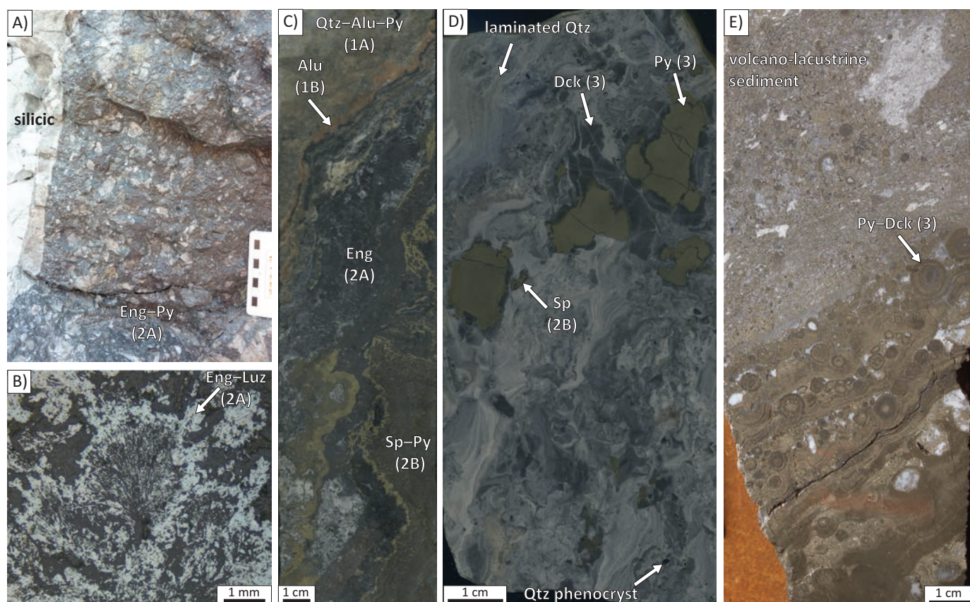
Fig. 6. Photographs and photomicrographs of selected ore textures from Mt. Carlton. (A) Silicic hydrothermal breccia cemented by stage 2A enargite-pyrite mineralization (from V2 pit). (B) Skeletal aggregates of stage 2A enargite and luzonite from A39 pit (reflected light, plane polarized; cf. Dekov et al., 2016, fig. 3). (C) Composite vein from V2 pit, illustrating part of the temporal sequence of alteration and mineralization at Mt. Carlton. A stage 1A quartz-alunite-pyrite-altered rhyodacite porphyry is crosscut by a stage 1B plumose alunite vein. The alunite vein served as a pathway for later mineralizing liquid, which deposited stage 2A enargite ore and, subsequently, stage 2B sphalerite-pyrite ore. (D) Sedimentary ore from A39 pit. The sediments are predominantly made up of finely laminated quartz. The siliceous sediments incorporated mineralized material from stage 2A (fine grained in photo), stage 2B, and stage 3, as well as volcanic sediment in the form of quartz phenocrysts. (E) Layered massive sulfide mineralization consisting of spherulitic stage 3 pyrite and dickite, within volcano-lacustrine sediment (unit 4A; from southwest corner of V2 pit). Abbreviations from Figure 3, and Eng = enargite, Luz = luzonite, Sp = sphalerite.
