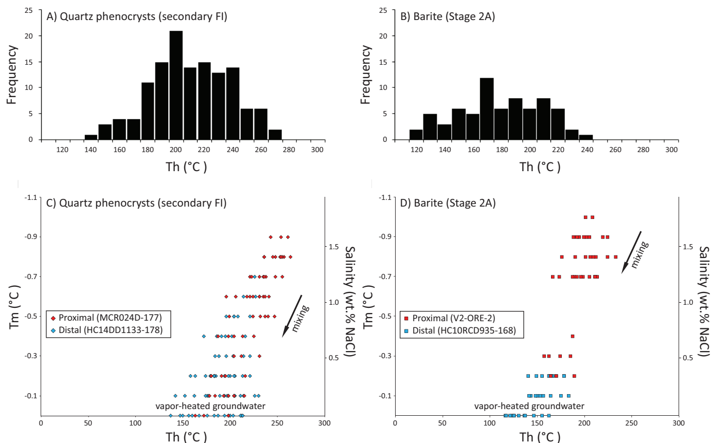
Fig. 9. Plots of fluid inclusion (FI) data. (A) Frequency histogram of homogenization temperatures (Th) of secondary fluid inclusions in quartz phenocrysts. (B) Frequency histogram of Th of primary fluid inclusions in barite associated with stage 2A mineralization. (C) Homogenization temperature (Th) versus final ice melting temperature (Tm) plot of secondary fluid inclusions in quartz phenocrysts. (D) Th versus Tm plot of primary fluid inclusions in barite. The observed Th versus Tm trends are interpreted to reflect mixing between low-salinity, magmatic-derived hydrothermal fluids and vapor-heated groundwater (~150°C, nil salinity). See text for detailed explanation.
