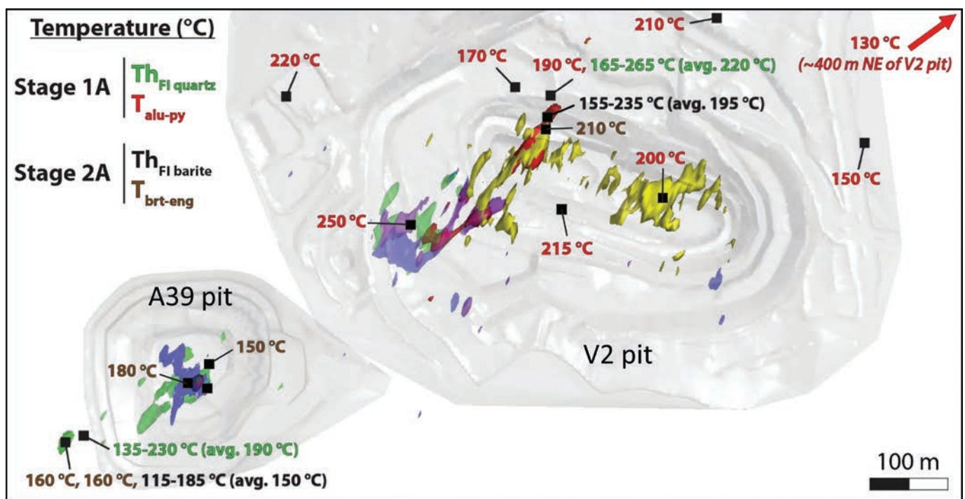
Fig. 8. Map of the Mt. Carlton open pits (cf. Fig. 2), showing the surface projections of samples used for geothermometry. Homogenization temperatures (Th) for fluid inclusions in quartz and barite and temperatures calculated from \Delta\delta^{34}\text{S}_{\text{sulfate-sulfide}} values are listed. All temperatures rounded to the nearest 5°C. Sample HC09DD025-120 (alunite-pyrite; A39 pit) is shown, but not annotated, due to the unrealistically high calculated equilibrium temperature of this distal sample (330°C). Abbreviations from Figure 3, and eng = enargite, FI = fluid inclusion.
