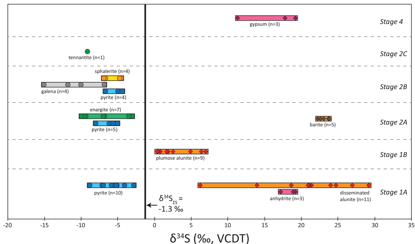
Fig. 10. Summary plot of \delta^{34}\text{S} values of sulfate, sulfide, and sulfosalt minerals.
