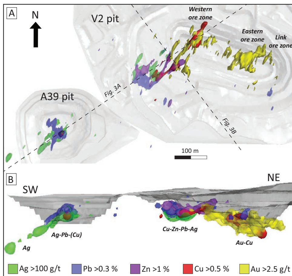
Fig. 2. 3-D model of the ore zones at Mt. Carlton, showing the zonation of Au, Cu, Zn, Pb, and Ag across the deposit. (A) Top view. The stippled lines indicate the surface traces of the sections shown in Figure 3. (B) Side view. Modified from Sahlström et al. (2018).
