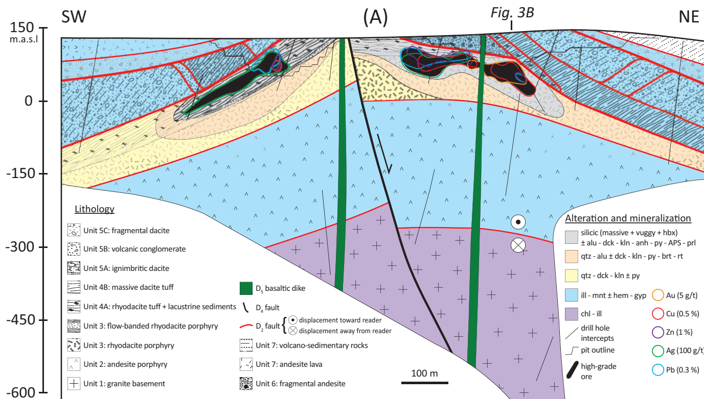
Fig. 3. Sections through Mt. Carlton, showing the distribution of stratigraphic units, major structures, alteration assemblages, and mineralization. (A) Northeast-southwest long section oriented parallel to the Western ore zone. (B) Northwest-southeast cross section through the southwest V2 pit. Abbreviations: alu = alunite, anh = anhydrite, APS = aluminium-phosphate-sulphate minerals, brt = barite, chl = chlorite, dck = dickite, gyp = gypsum, hbx = hydrothermal breccia, hem = hematite, ill = illite, kln = kaolinite, mnt = montmorillonite, prl = pyrophyllite, py = pyrite, qtz = quartz, rt = rutile. Modified from Sahlström et al. (2017, 2018).
