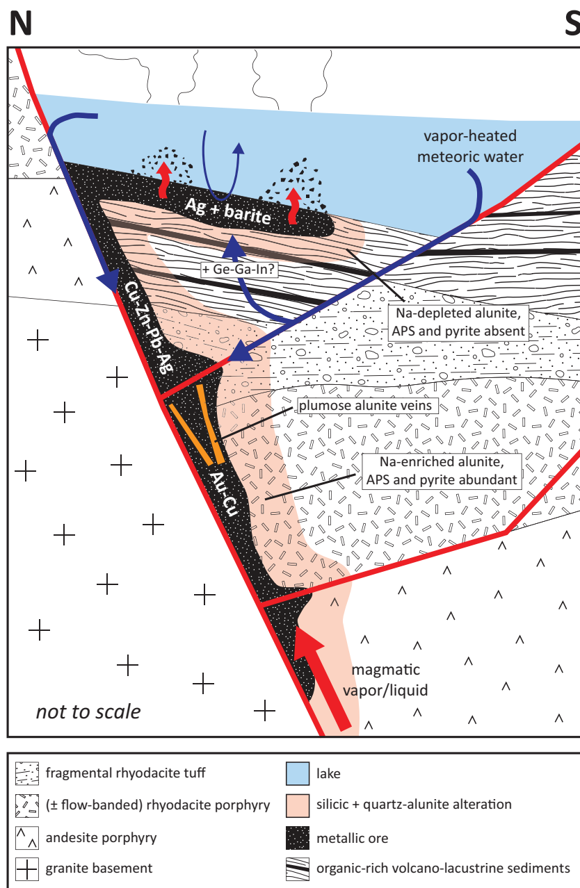
Fig. 12. Conceptual genetic model for Mt. Carlton, integrating geologic, structural, mineralogical, and geochemical data and observations (Sahlström et al., 2017, 2018; this study). Mt. Carlton formed in a shallow volcano-sedimentary rift environment, in a sublacustrine setting, where magmatic vapor initially condensed into meteoric water, followed by magmatic liquid diluted by meteoric water. See text for detailed explanation.
