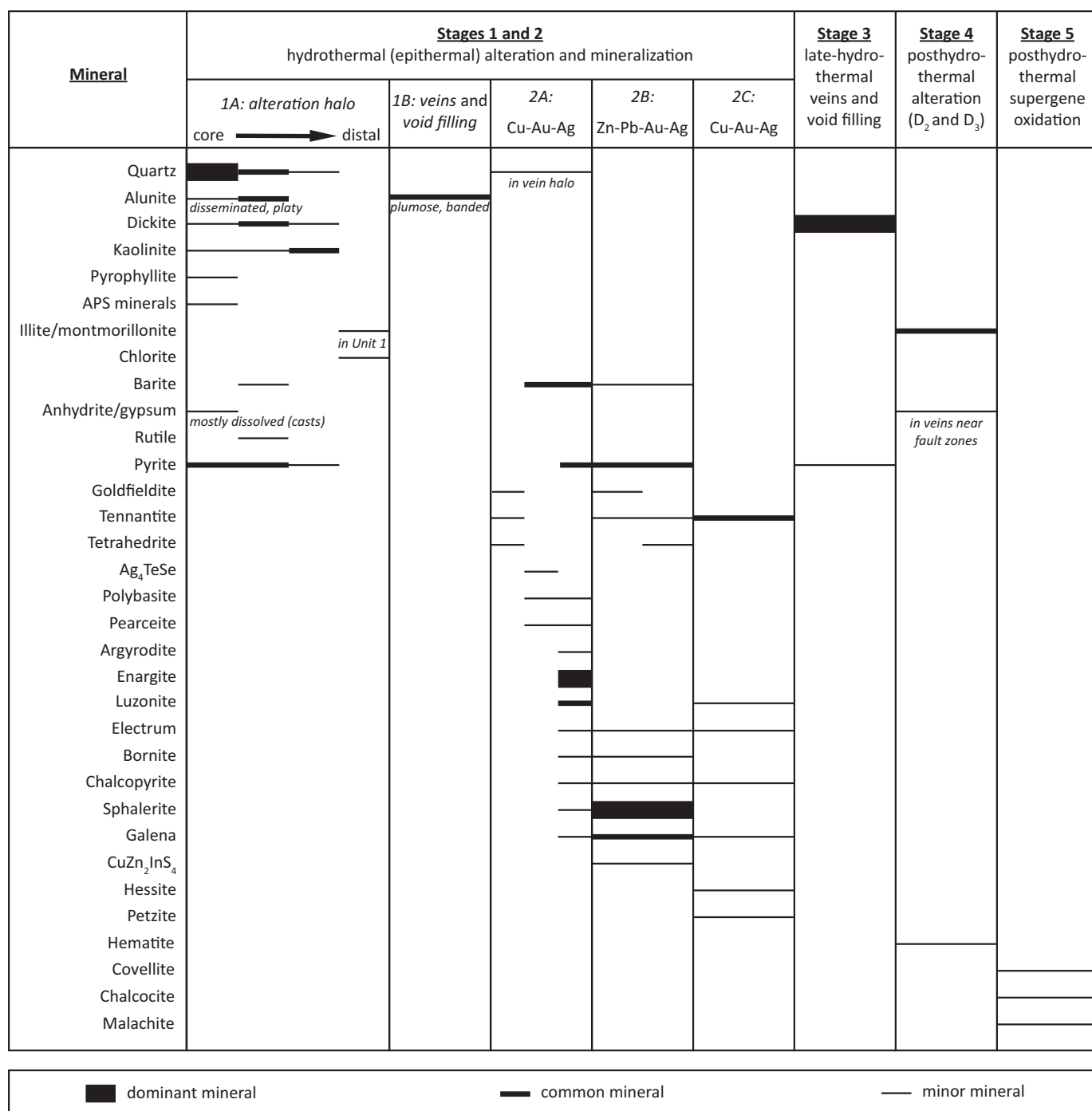
Fig. 4. Paragenetic sequence of alteration and ore minerals at Mt. Carlton. Modified from Sahlström et al. (2018).
