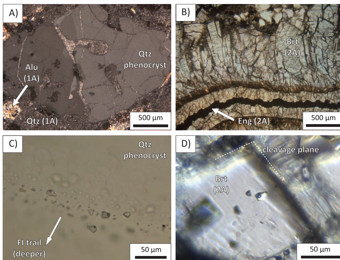
Fig. 7. Photomicrographs of the studied fluid inclusion assemblages from Mt. Carlton. (A) Igneous quartz phenocryst in a hydrothermally altered quartz-feldspar-phyric rhyodacite. The quartz crystal exhibits fractures and corrosion textures, which have been infilled with stage 1A quartz and alunit. Secondary fluid inclusions are locally developed in trails propagating from such fractures or from quartz crystal boundaries (transmitted light, cross polarized). (B) Coarse-grained, euhedral barite crystals occurring in the halo of a stage 2A enargite veinlet. The barite crystals grew perpendicular to the enargite veinlet and contain both primary and secondary fluid inclusions (transmitted light, plane polarized; see Sahlström et al., 2017, fig. 4E). (C) Trail of secondary fluid inclusions developed within an igneous quartz phenocryst (transmitted light, plane polarized). (D) Primary fluid inclusion within a barite crystal associated with stage 2A enargite mineralization (transmitted light, plane polarized). Abbreviations from Figure 3, and Eng = enargite, FI = fluid inclusion.
