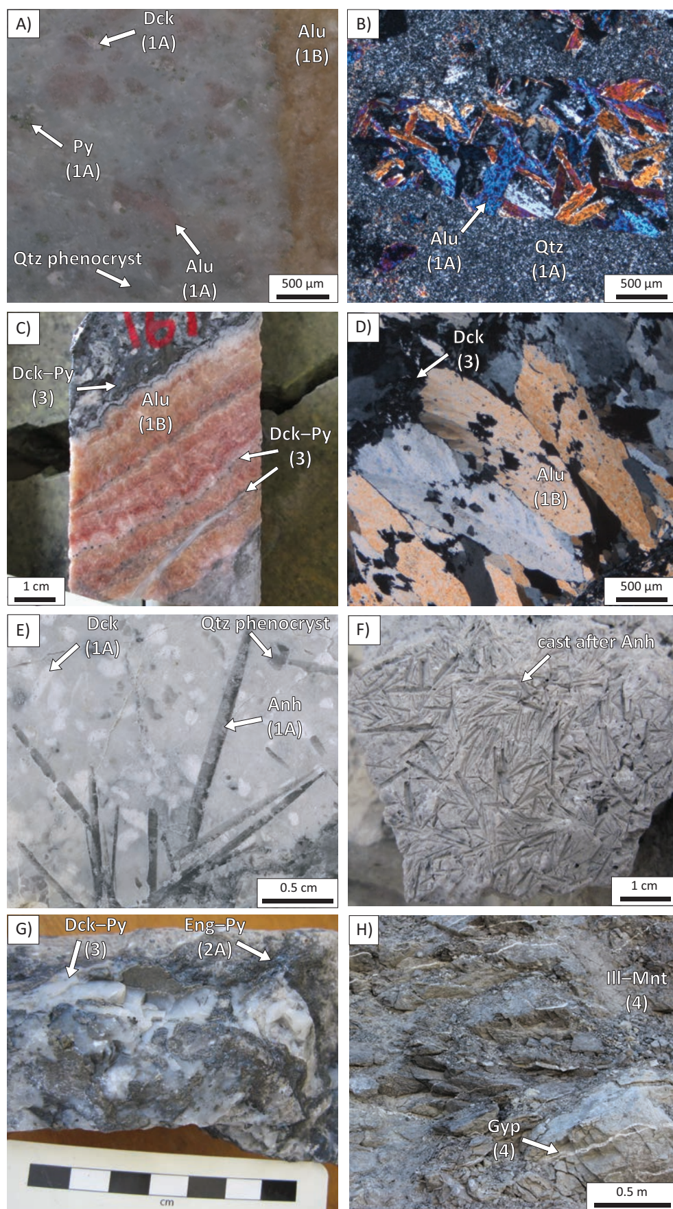
Fig. 5. Photographs and photomicrographs of selected alteration assemblages from Mt. Carlton. (A) Stage 1A quartz-alunite-dickite-pyrite alteration developed in a quartz-feldspar-phyrlic rhyodacite (unit 3). The stage 1A assemblage is crosscut by a younger stage 1B plumose alunite vein. (B) Aggregate of stage 1A alunite crystals that have replaced a preexisting feldspar crystal (transmitted light, cross polarized). (C) Stage 1B banded, plumose alunite vein. The alunite vein has locally been overprinted by stage 3 dickite-pyrite veinlets. (D) Plumose texture in a stage 1B alunite vein (transmitted light, cross polarized). (E) Aggregate of tabular stage 1A anhydrite crystals developed within open space in a silicified altered rhyodacite porphyry. (F) Alteration similar to that in (E) but with the anhydrite having been completely dissolved, leaving behind distinctive casts in the rock. (G) Stage 2A enargite-pyrite mineralization overprinted by void fill made up of stage 3 massive dickite with pyrite. (H) Stage 4 illite-montmorillonite alteration developed in a massive dacite tuff (unit 4B) in the northern wall of V2 pit. Veins made up of fibrous gypsum with a well-developed shear fabric occur near a D 2 fault zone. Abbreviations from Figure 3, and Eng = enargite.
